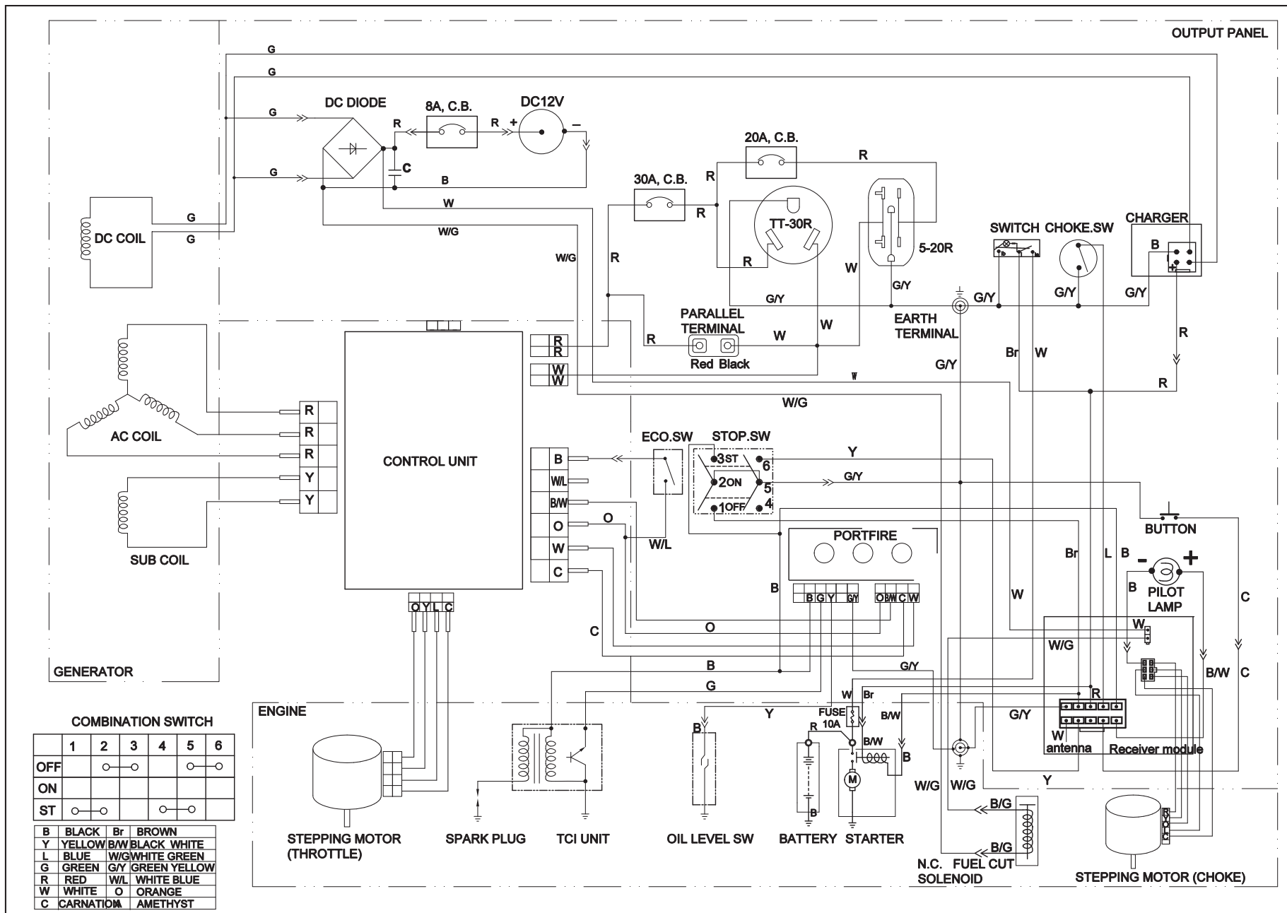
Wiring Diagram
