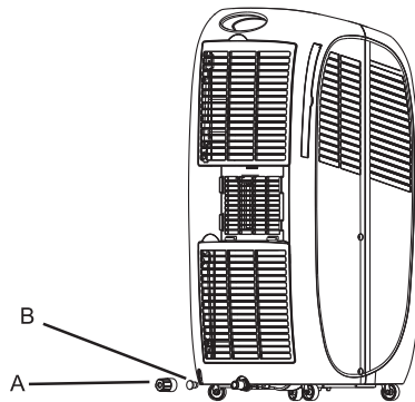
A. Primary drain cover B. Primary drain plug
