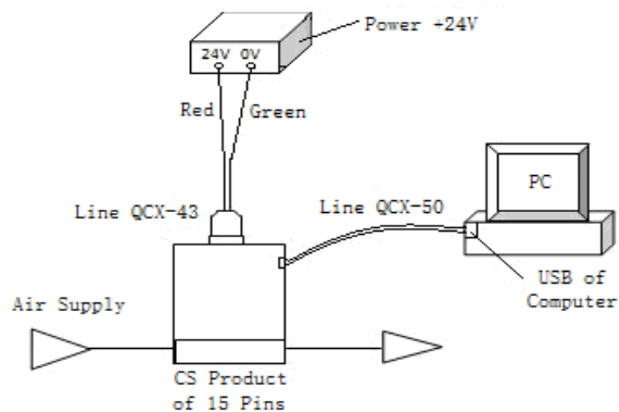
Figure 2-19 CS Product and Illustration of Connecting Power
