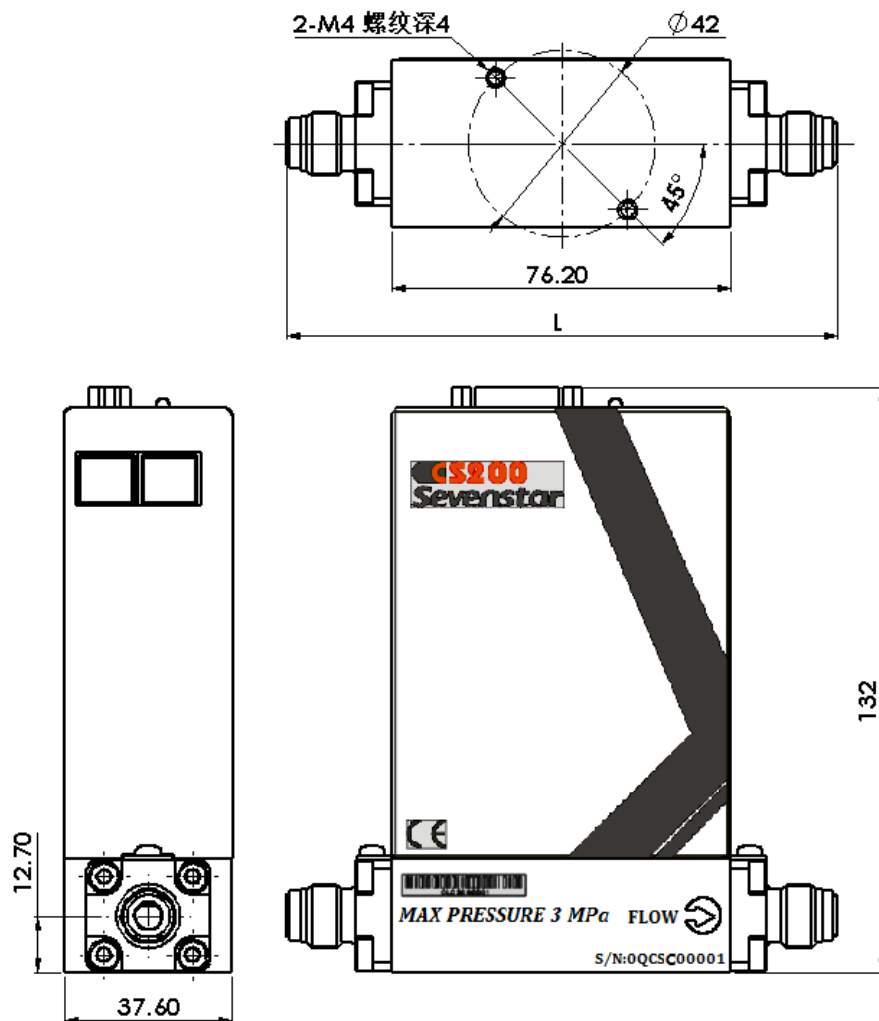
Figure 2-2 Product dimensions
