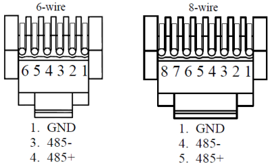
Figure 2-11 RS485 connector
