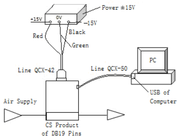
Figure 2-18 CS Product and Illustration of Connecting Power
