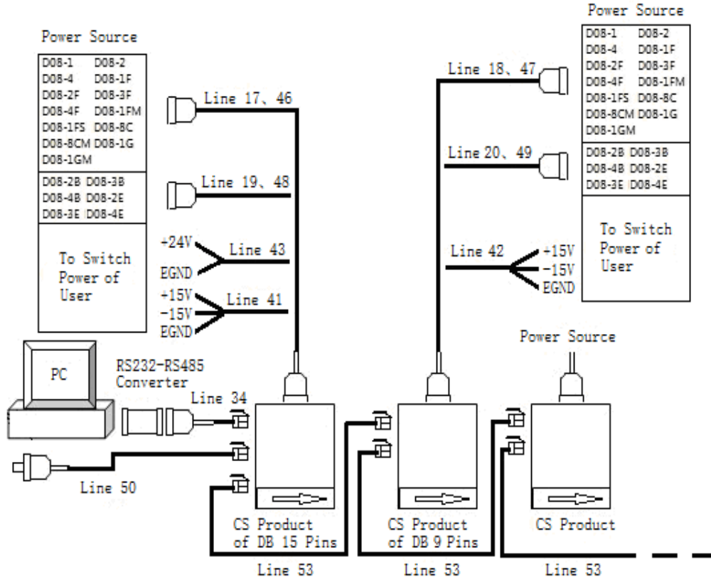
Figure 2-20 Illustration of Connecting CS Product
