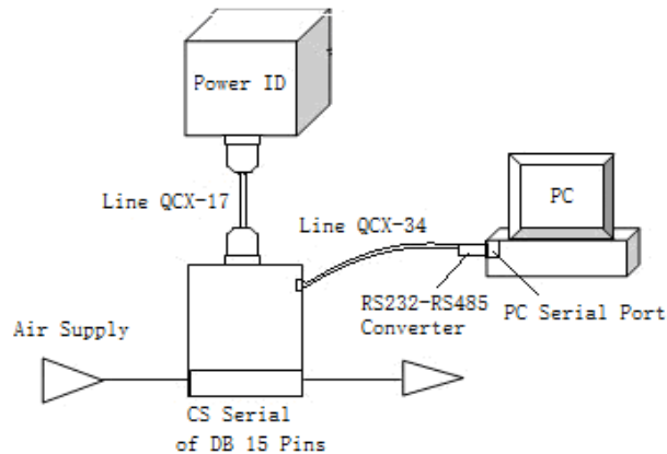
Figure 2-17 CS Product and Illustration of Connecting Power D08-1D/1F
