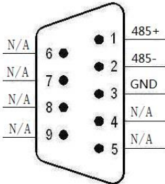
Figure 2-14 RS232-RS485 connector
