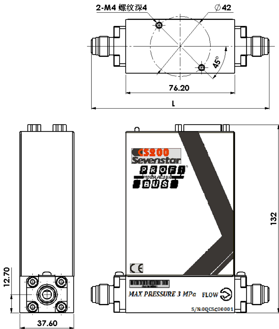
Figure 2-4 Product dimensions
