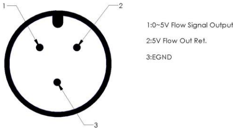
Figure 2-13 Analog Signal Interface
