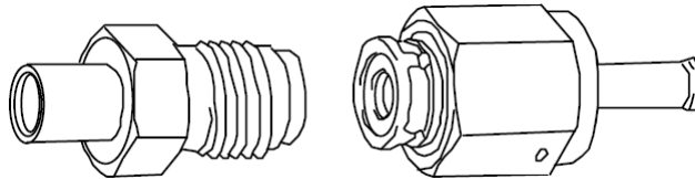
Figure 2-7 VCR retainer gasket
