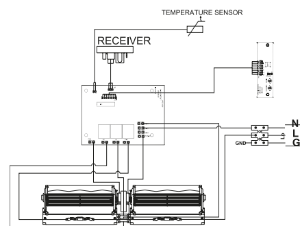
Figure 5: Electrical Wiring
