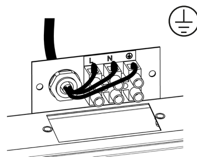
Figure 4: Electrical Connection
