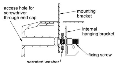
Figure 3: Cross Sectional View of Mounting Bracket
