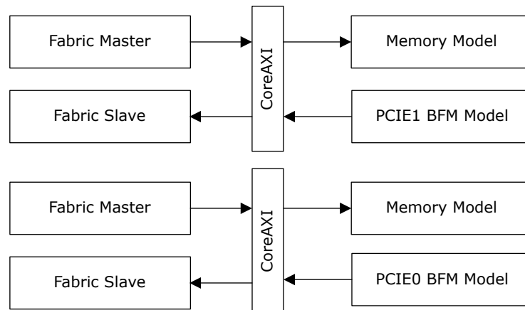
Figure 3-12. PCIESS BFM Structure
