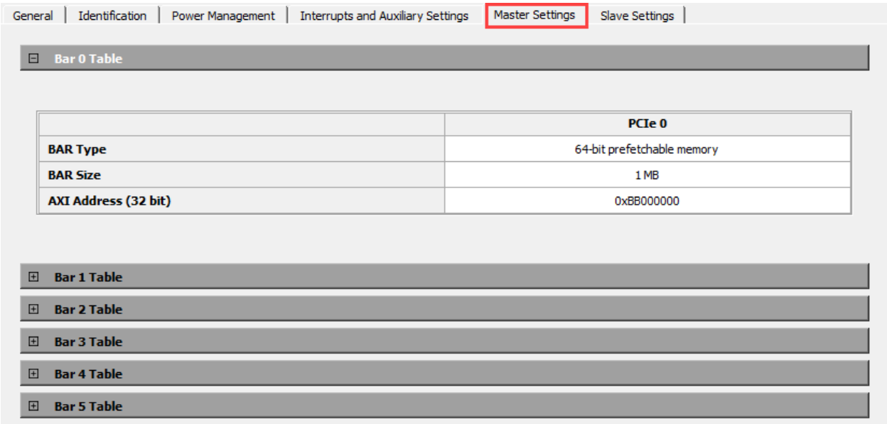
Figure 1-12. Example of Configuring Master RP Settings
