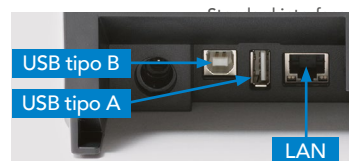
Interface options
