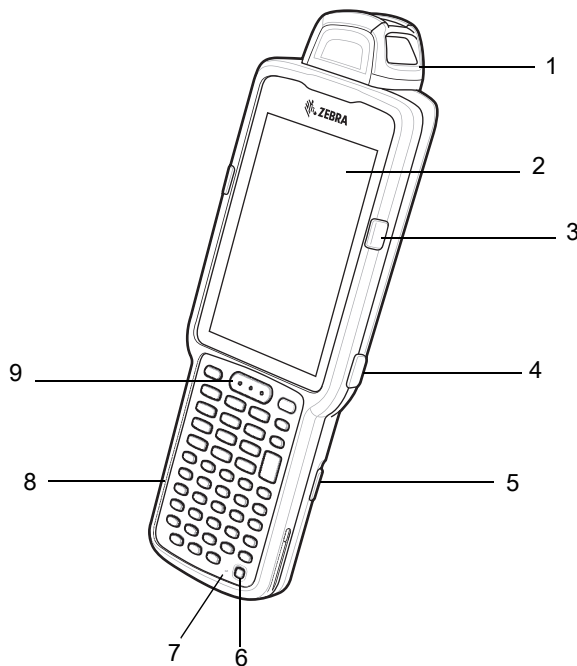
Figure 4 MC3300x-R Front View
