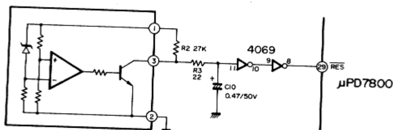
Fig. 18 Reset circuit
