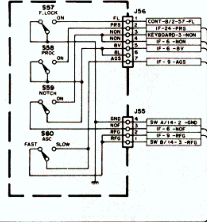
DISPLAY UNIT (X54-1870-00)(D/4)
