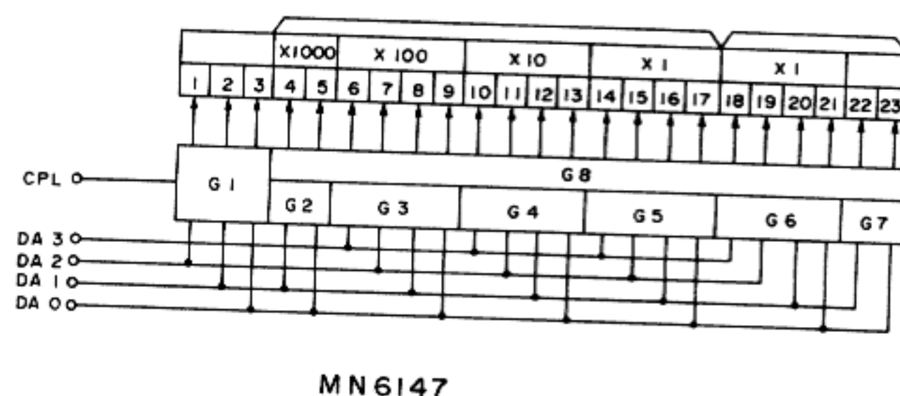
Fig. 20 Data input terminal and programmable counter
