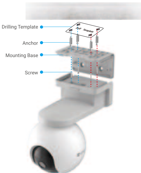
Fig. 1 Ceiling Mount
