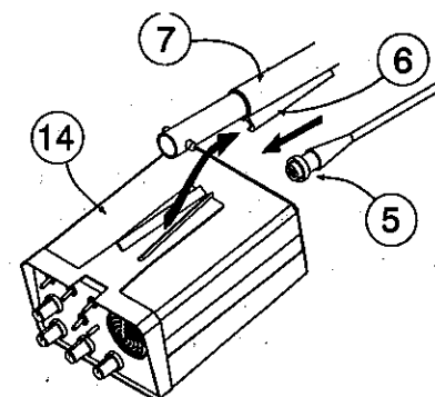
Figure 5 — Mounting the Control Box on the Shaft
