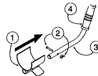
Figure 2 — The Armrest and Upper Shaft Assembly
