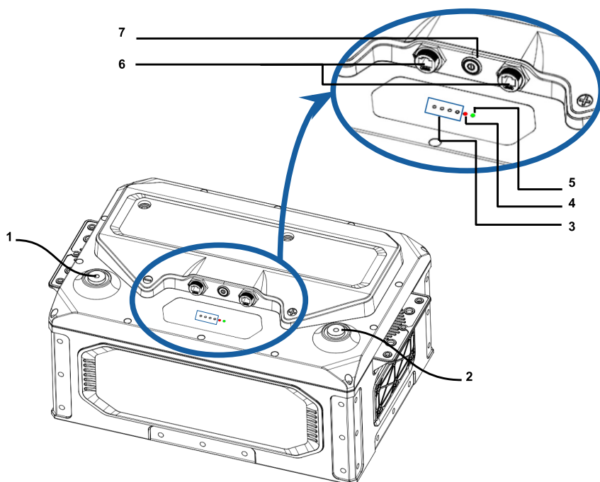
Figure 2: HUSKY 2 Battery Diagram
