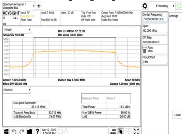
802.11ax_40MHz_Chain0_7005MHz
