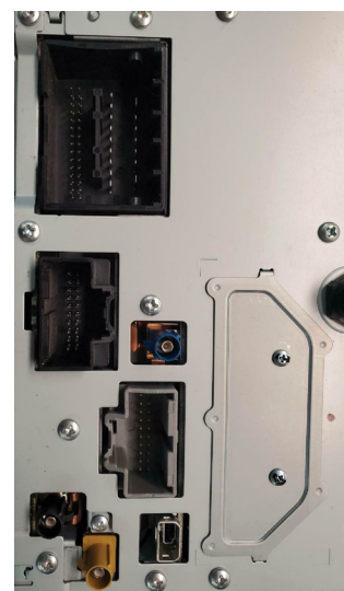
Back View of Car Navigation
