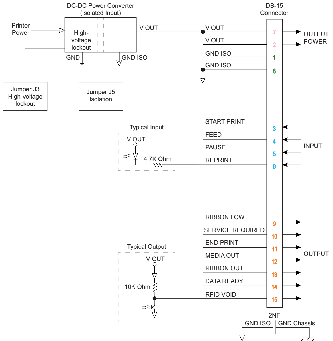
Figure 10 External Pinouts
