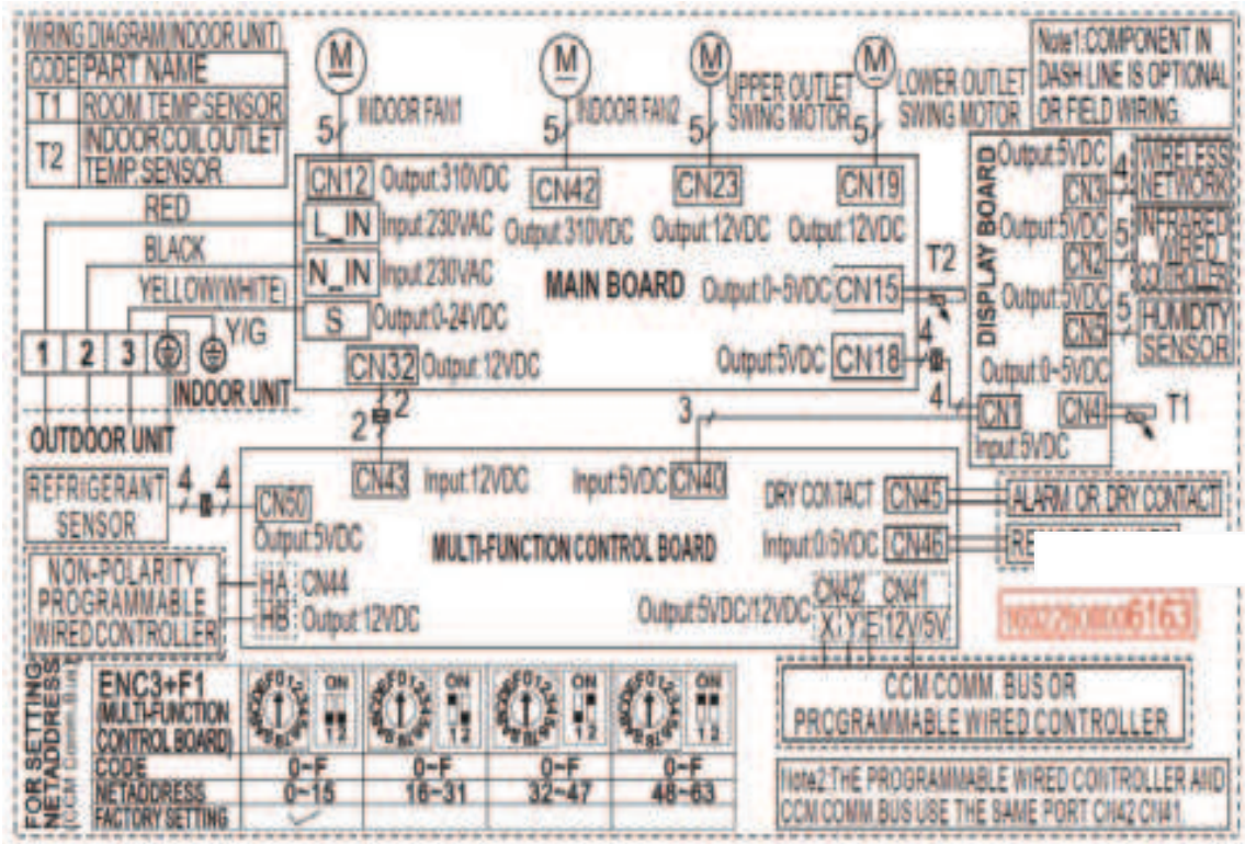
Fig. 15 – Wiring Diagram Sizes 09K, 12K, 16
