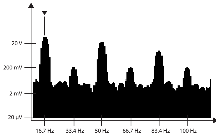
Figure 2-13: Interference in railroad environment (rated frequency at 16.7 Hz)
