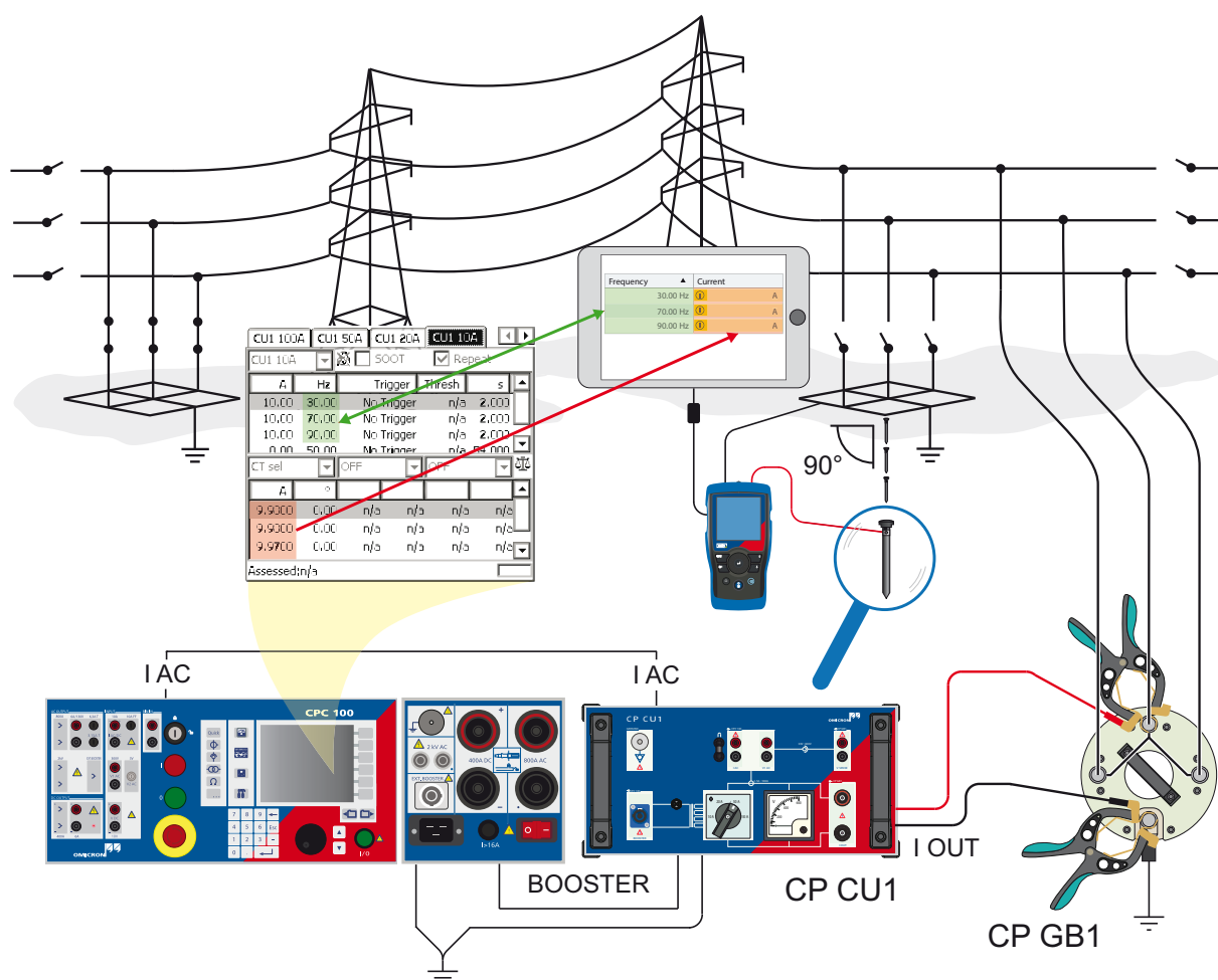
Figure 5-11: Ground impedance measurement setup when using PTM on a tablet
