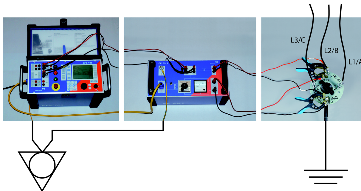
Figure 3-3: CP CU1 measurement setup with CPC 100 and CP GB1
