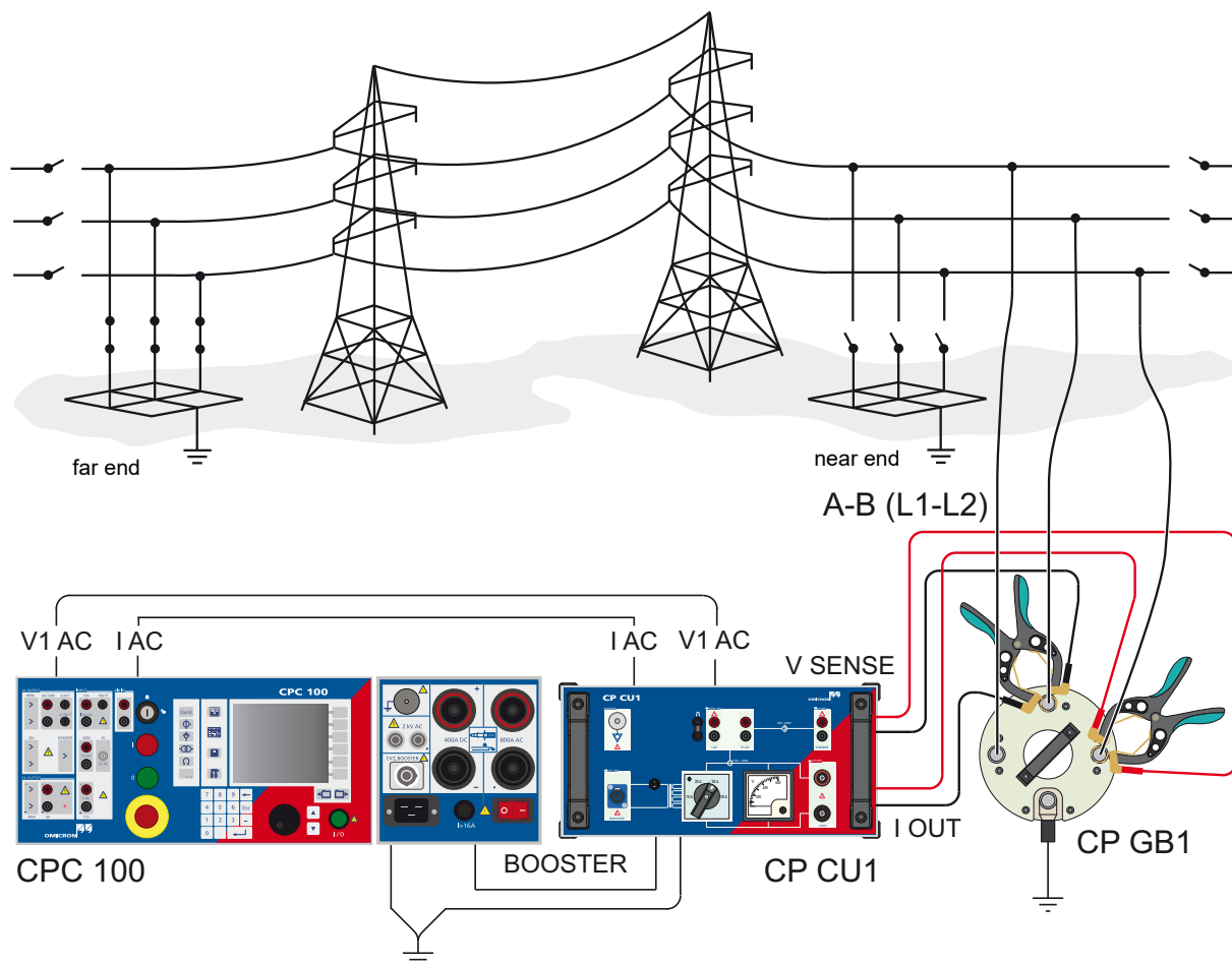
Figure 4-8: Line impedance measurement loop A-B (L1-L2)
