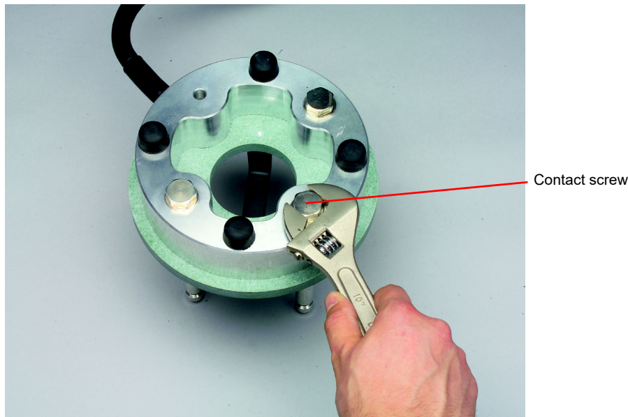
Figure 2-10: Opening the surge arrestor chamber
