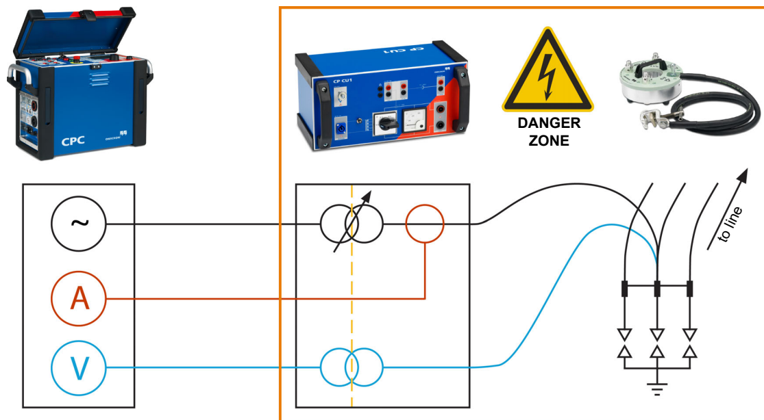
Figure 2-12: Test setup consisting of CPC 100, CP CU1 and CP GB1.
