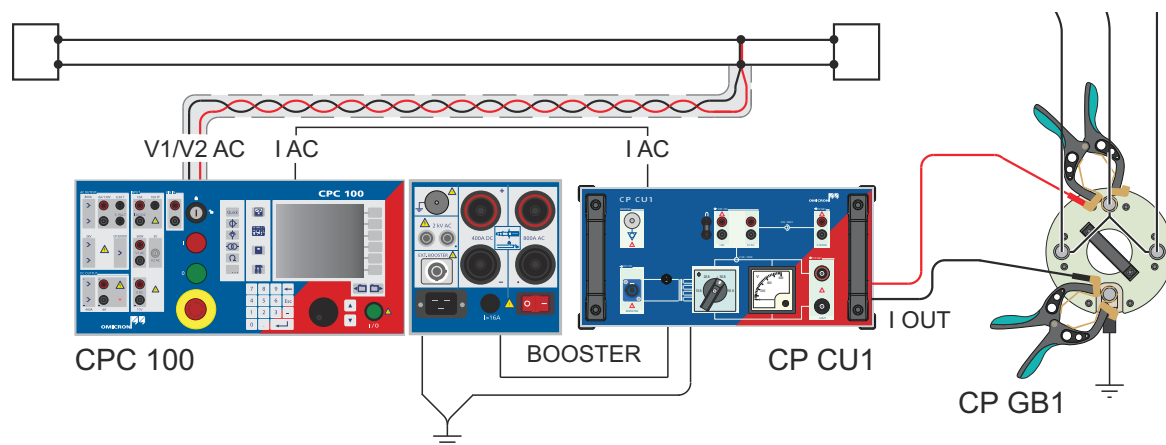
Figure 6-4: Coupling into signal cables measurement setup for the line-to-ground calibration
