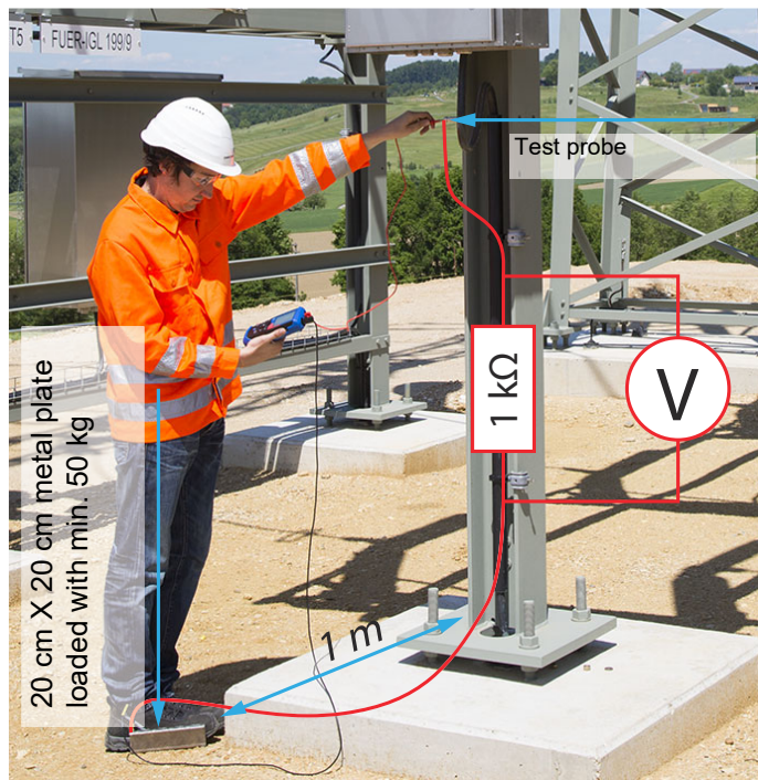
Figure 5-19: Touch voltage measurement according to EN 50522
