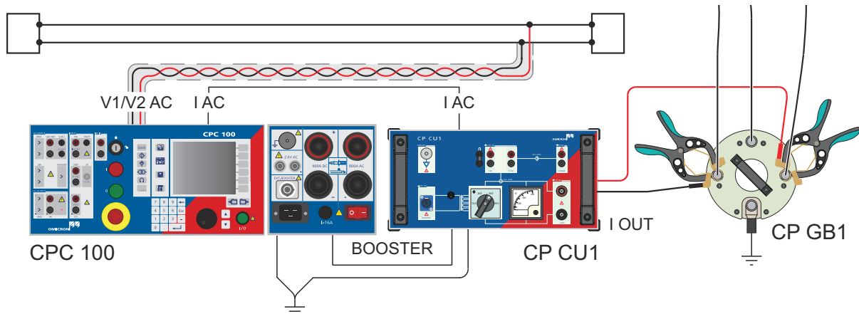
Figure 6-2: Coupling into signal cables measurement setup for the line-to-line measurement
