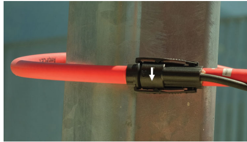
Figure 5-31: Example: Three return currents - three measurements
