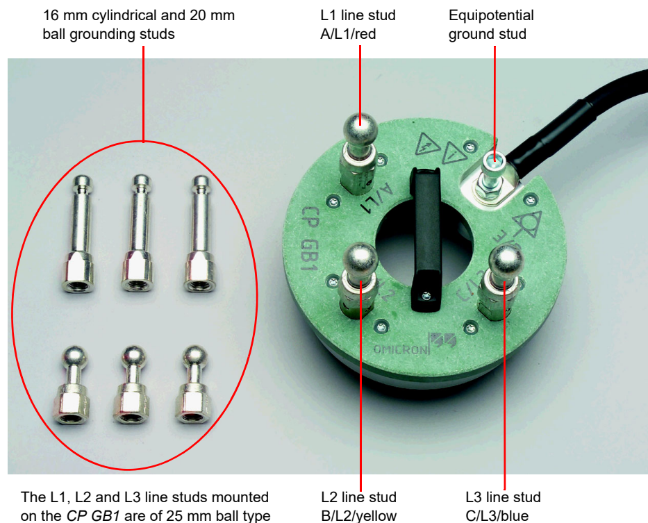
Figure 2-3: CP GB1 grounding box
