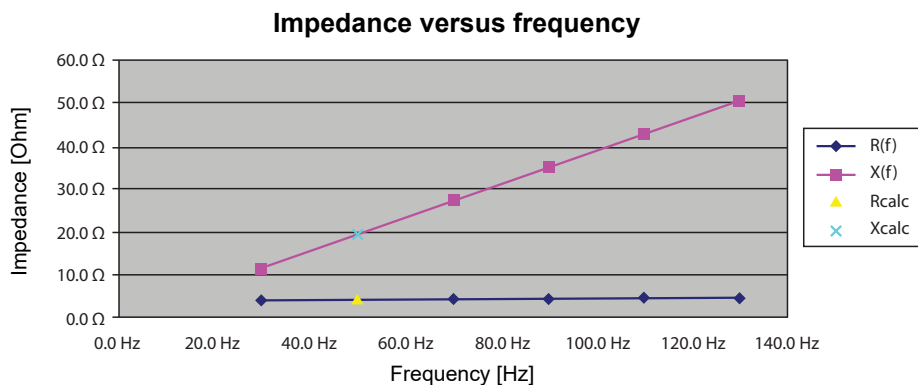
Figure 2-15: Interpolation to rated frequency
