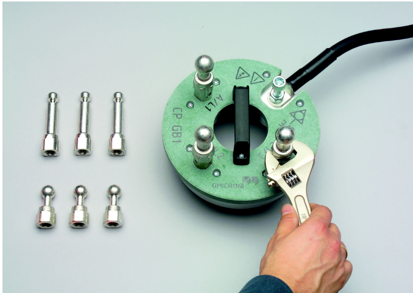
Figure 2-5: Screwing on the CP GB1 's grounding studs
