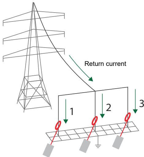
Figure 5-31: Example: Three return currents - three measurements
