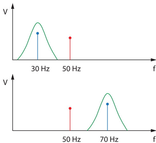
Figure 2-14: Frequency-selective measurement
