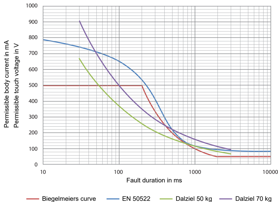
Figure 5-4: Permissible body currents from EN 50522 and IEEE 80
