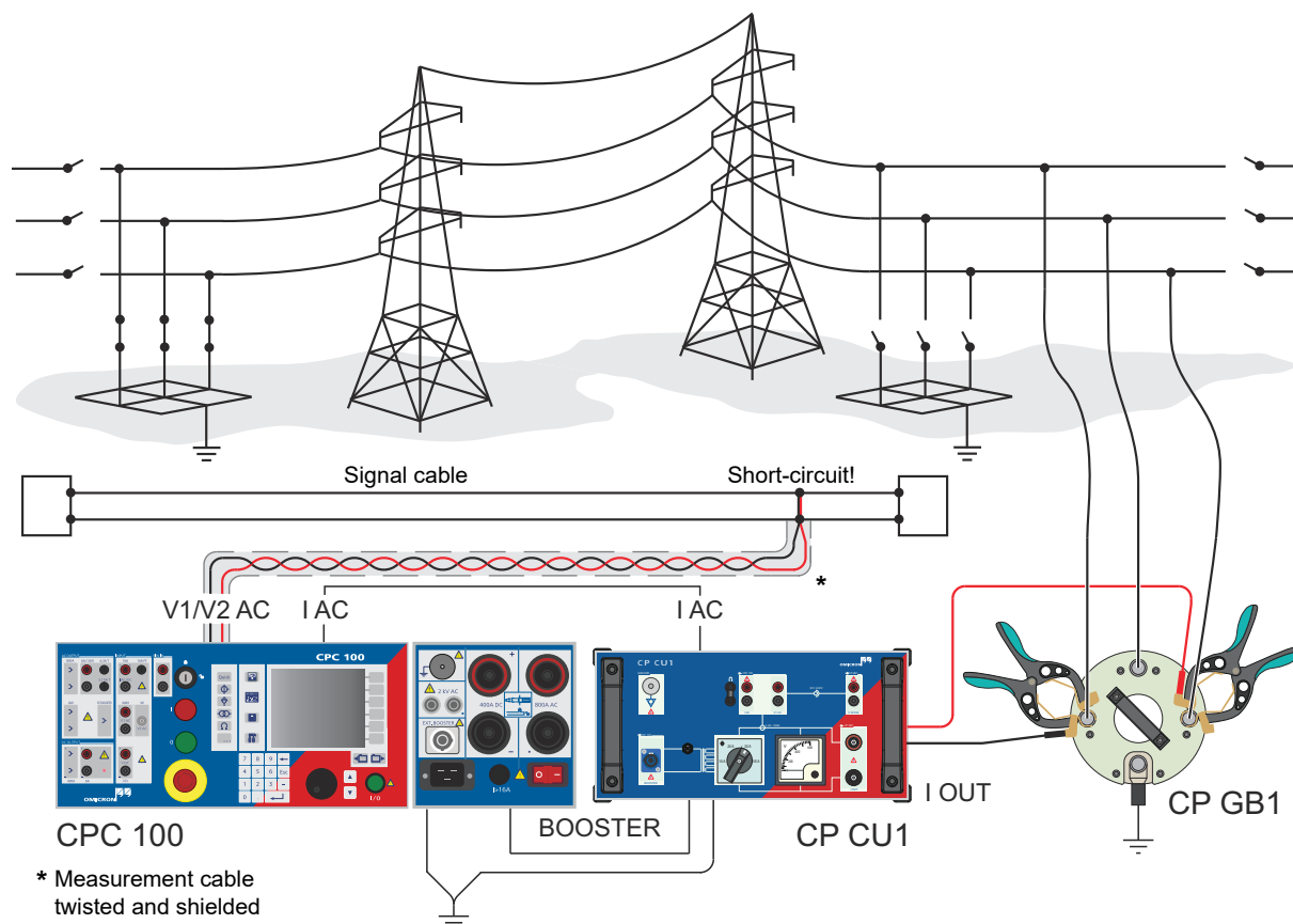
Figure 6-1: Coupling into signal cables measurement setup for the line-to-line calibration
