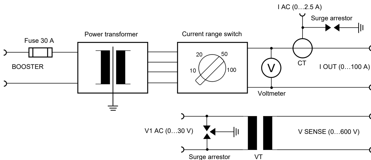
Figure 2-1: Circuit diagram of the CP CU1
