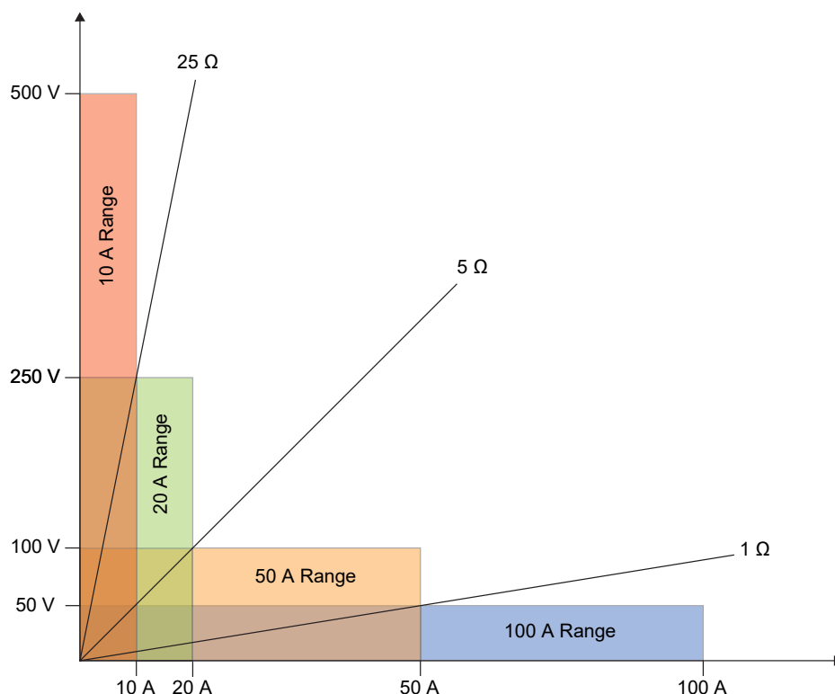
Figure 2-16: Load diagram of the CP CU1
