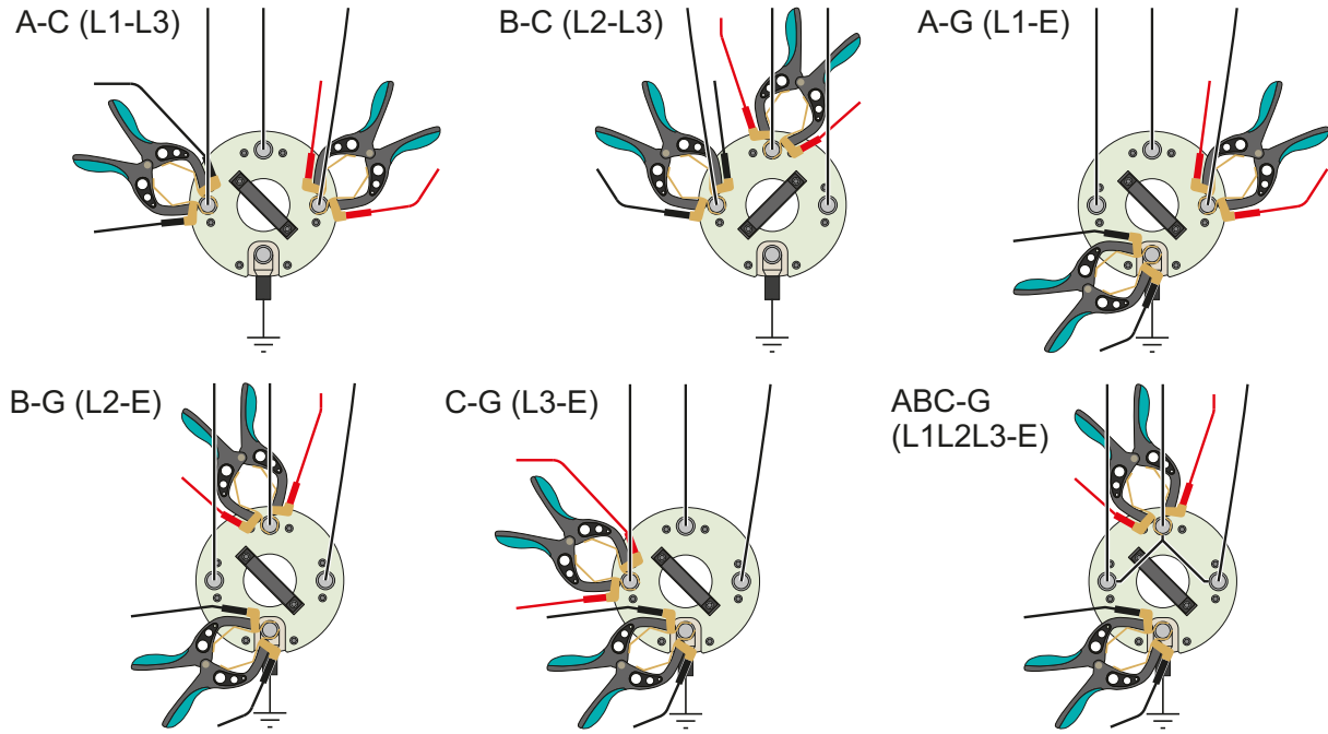
Figure 4-9: Clamp connections for measurement loops 2 to 7
