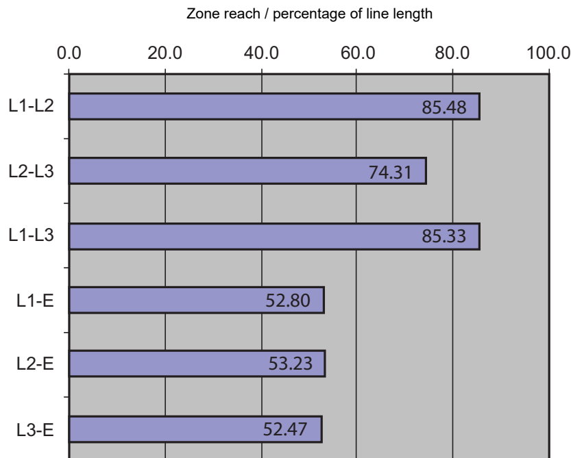
Figure 4-2: Zone reaches
