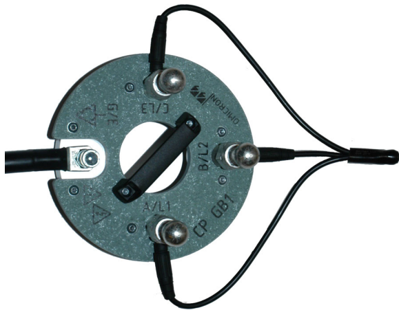
Figure 2-7: Shorting the phases
