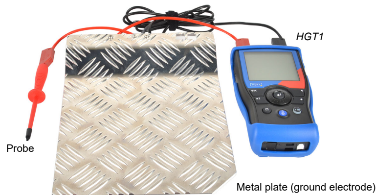
Figure 5-27: HGT1 hardware setup according to EN 50522
