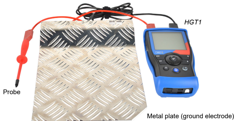
Figure 5-21: HGT1 hardware setup according to EN 50522
