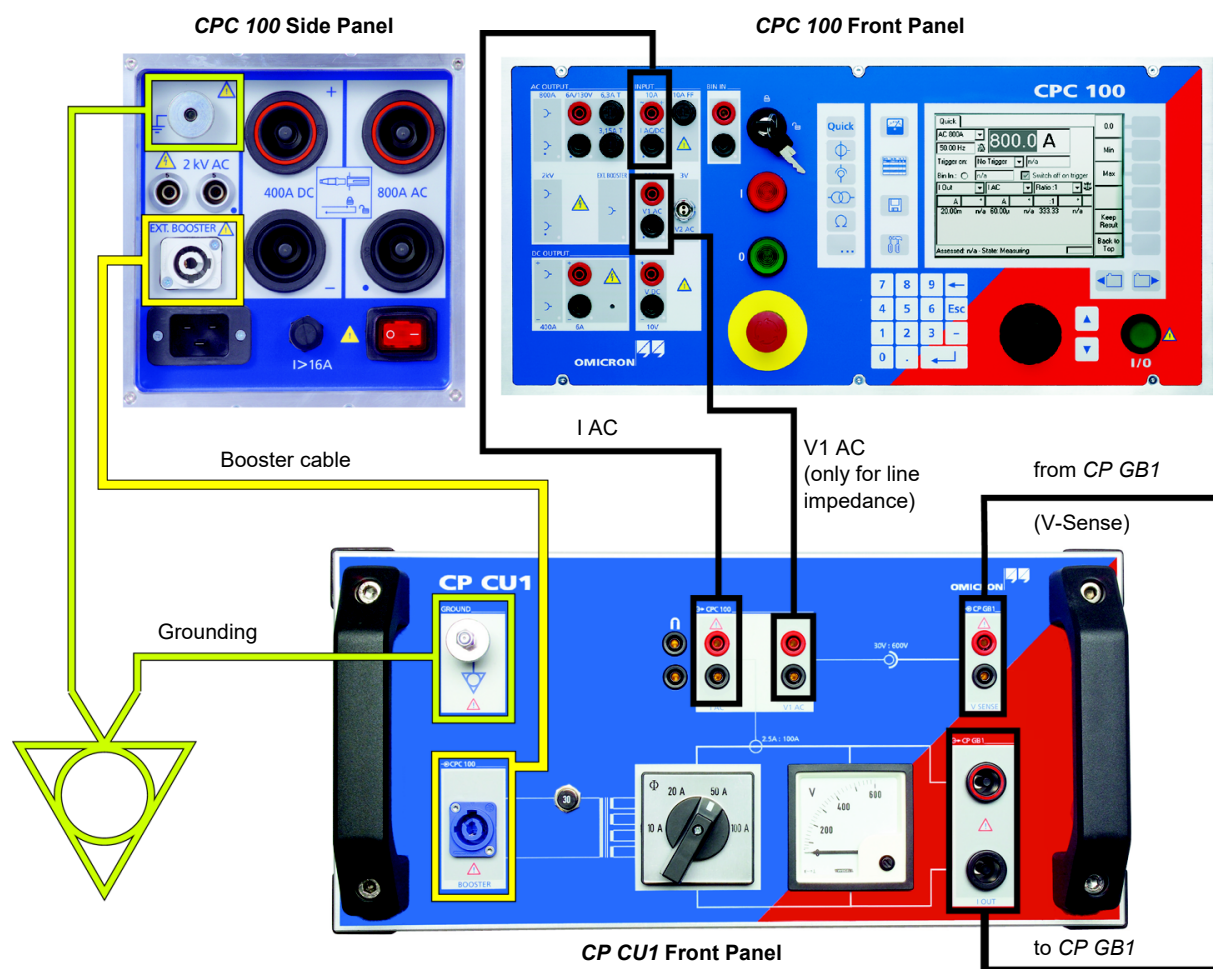
Figure 3-4: Connecting the CPC 100 to the CP CU1
