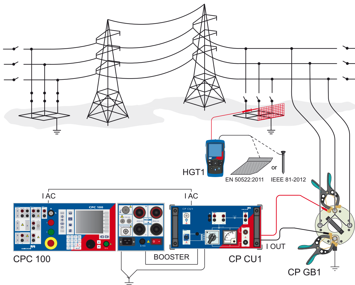
Figure 5-15: Step and touch voltage measurement setup
