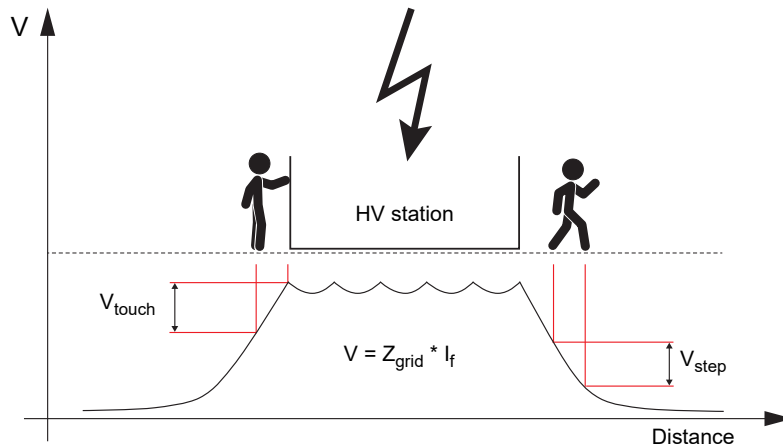
Figure 5-3: Step and touch
