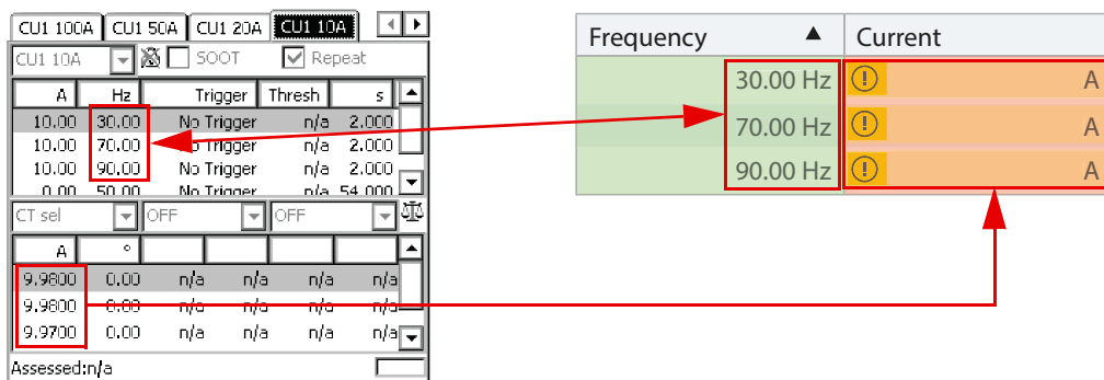
Figure 5-14: Enter the current readings under the Settings and Conditions section in PTM
