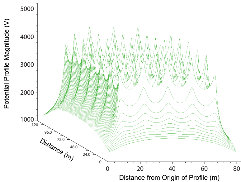
Figure 5-2: Potential contours of a ground grid
