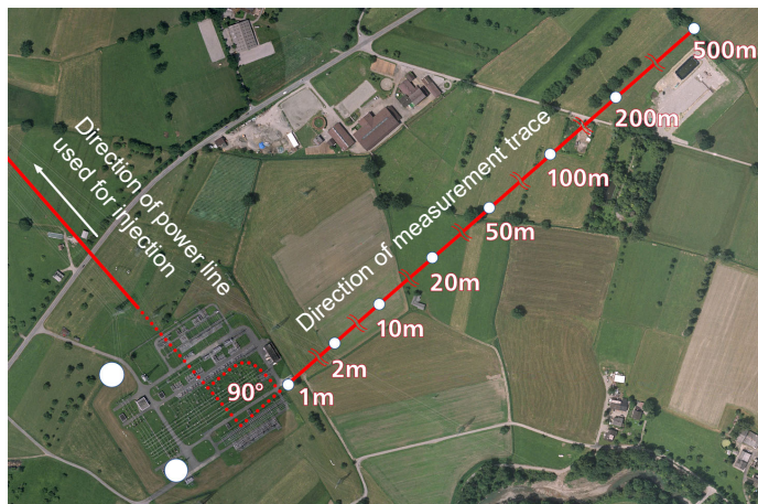
Figure 5-12: Direction of measurement trace
