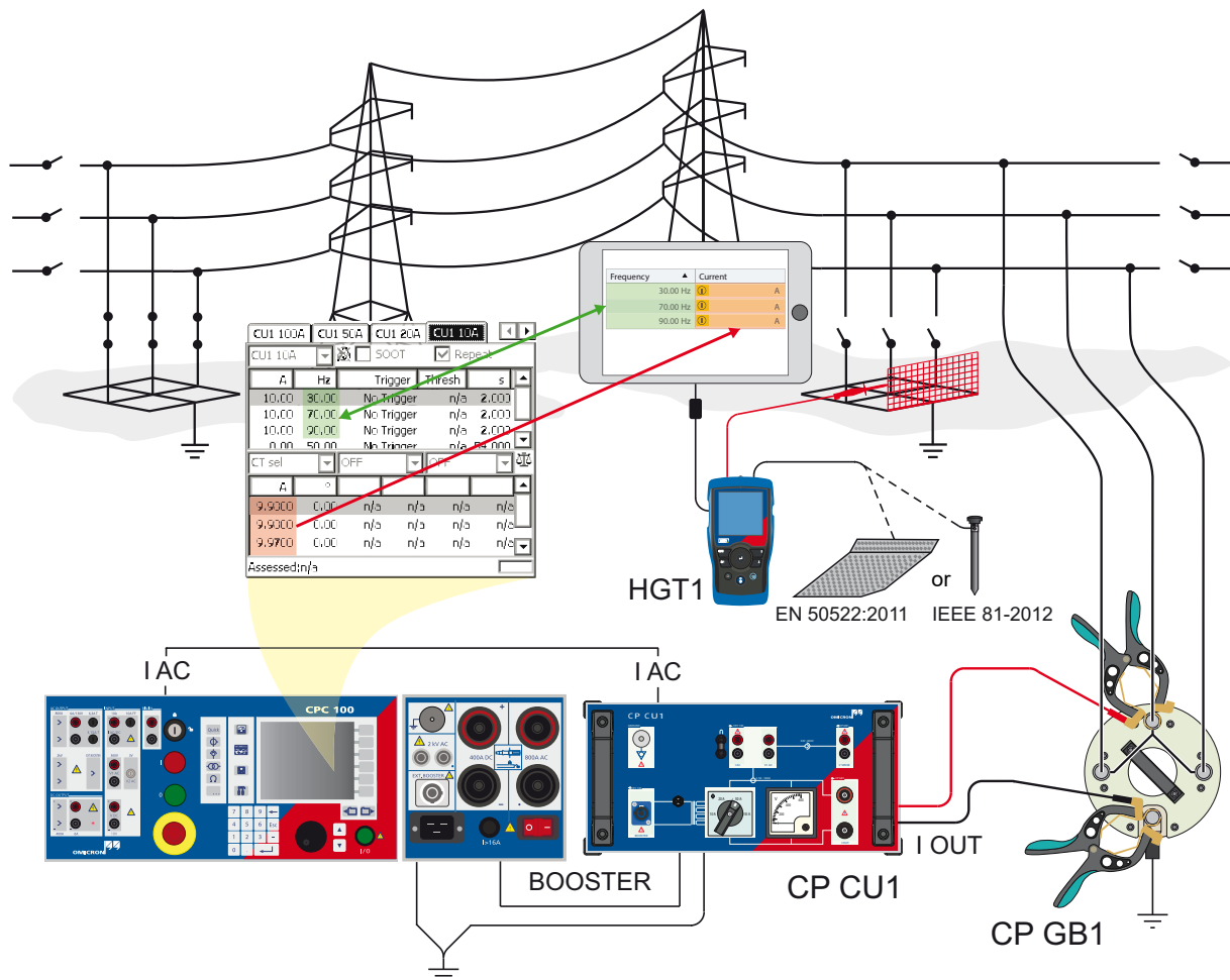
Figure 5-23: Step and touch voltage measurement setup when using PTM on a tablet
