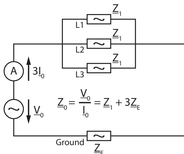
Figure 4-1: Zero-sequence impedance definition
