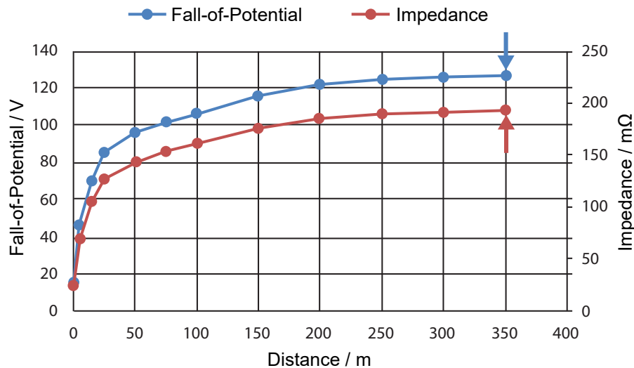
Figure 5-10: Impedance and voltage profile
