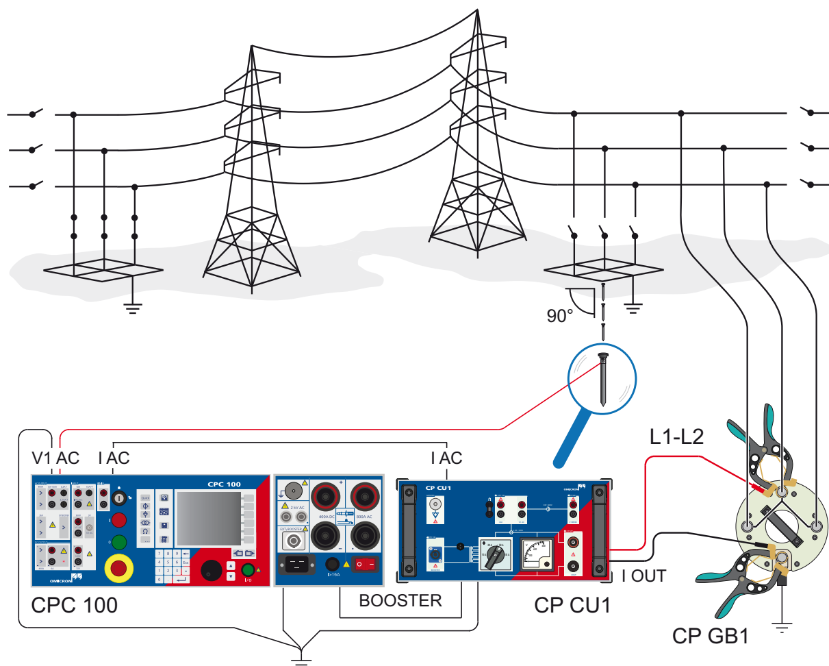
Figure 5-5: Ground impedance measurement setup
