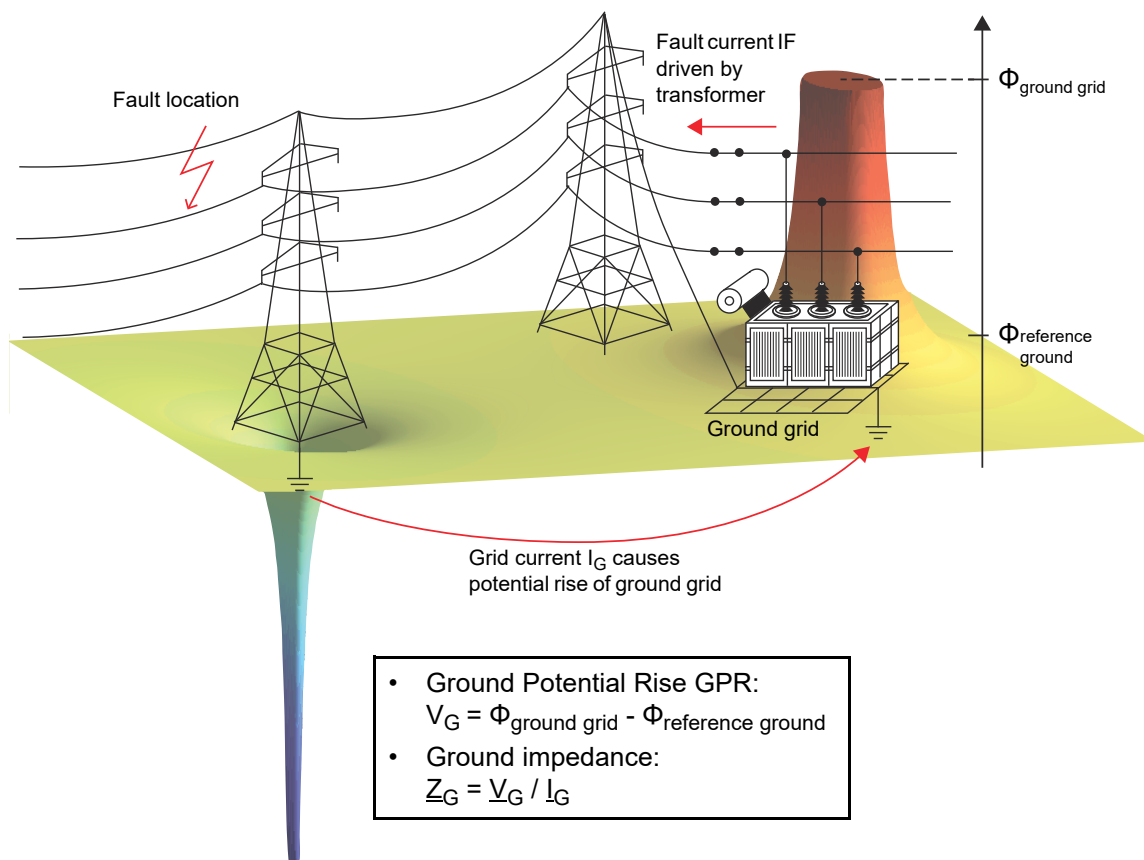
Figure 5-1: Potential during a ground fault
