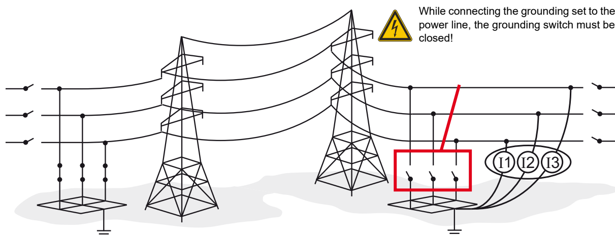
Figure 3-1: Estimating the open-line voltage
