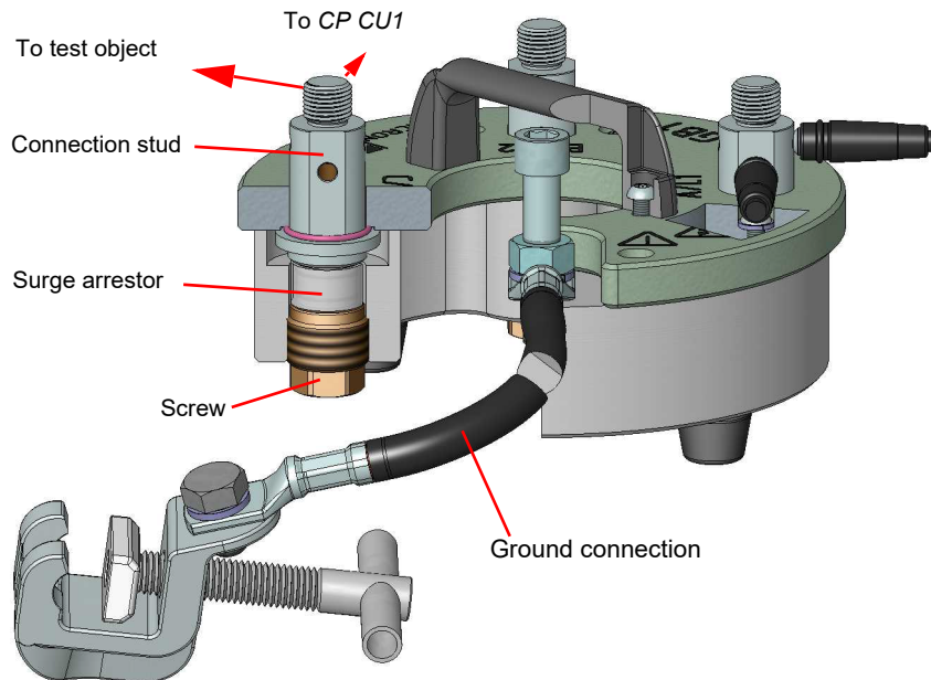
Figure 2-4: Cross-sectional view of the CP GB1
