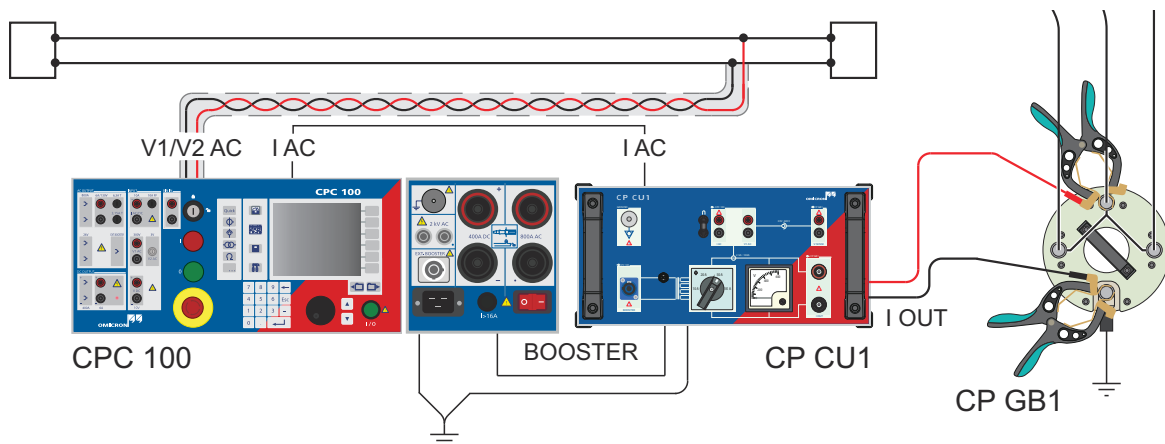
Figure 6-3: Coupling into signal cables measurement setup for the line-to-ground measurement
