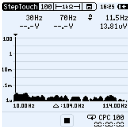
Figure 5-20: HGT1 settings according to EN 50522
