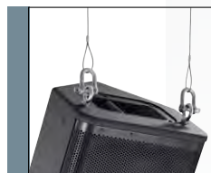
M10 rigging points for suspended installation (DSR115/DSR112).
