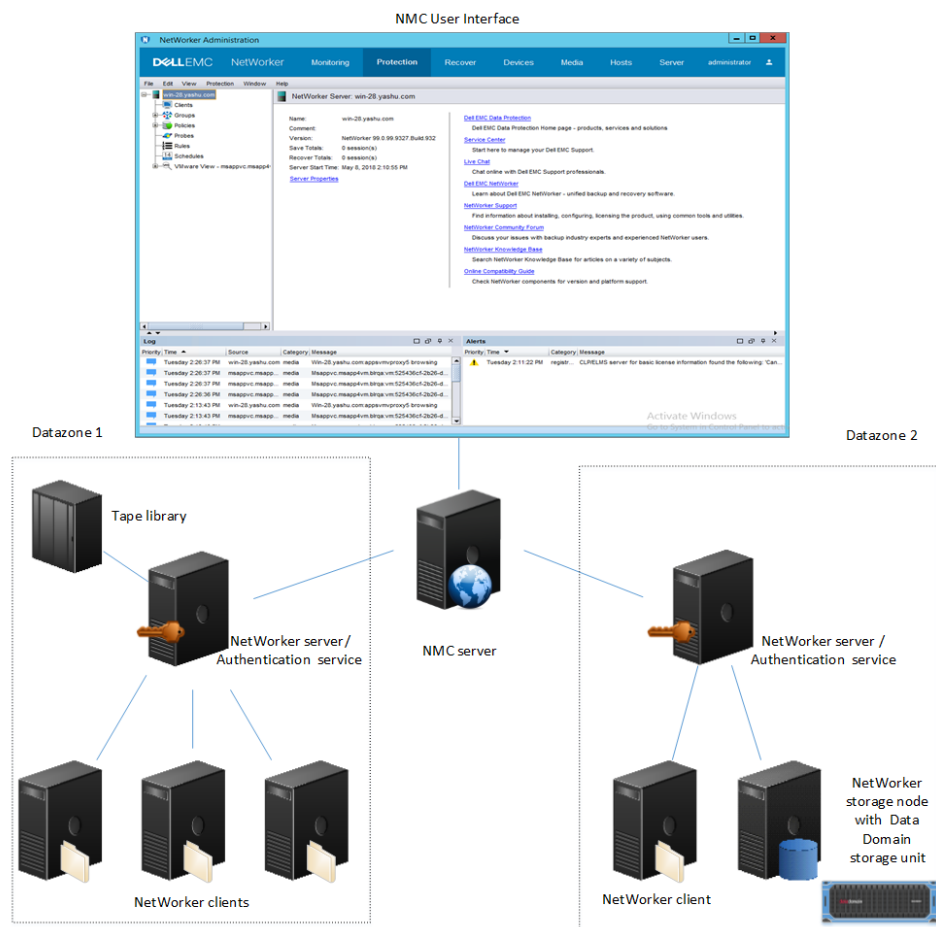
Figure 1 NetWorker components
