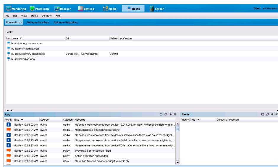
Figure 86 Hosts window
