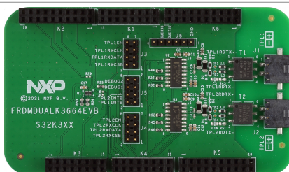
Figure 5. FRDMDUALK3664EBV transceiver board
