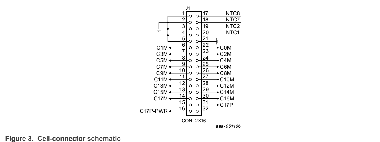
Figure 3. Cell-connector schematic
