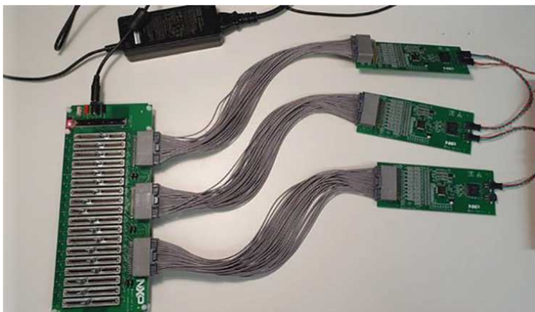
Figure 6. RD33774PDSTEBVs connection to a BATT-18EMULATOR
