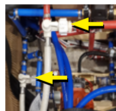
Aqua-Hot Bypass Valves
