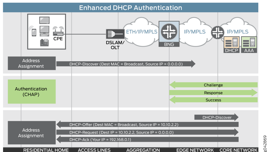
Figure 6: Enhanced DHCP Authentication
