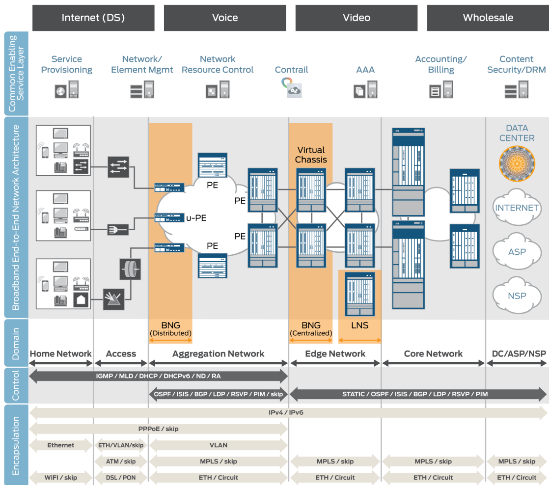
Figure 2: The Broadband Edge Architecture
