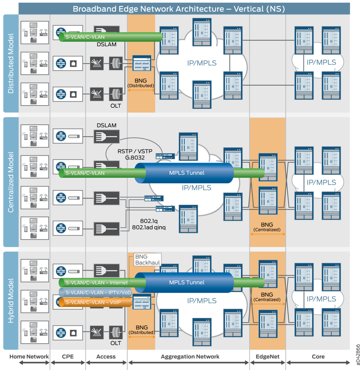
Figure 5: Broadband Edge Network Architectural Models
