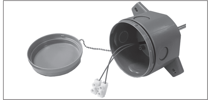
Figure 4.2 - Sensor Junction Box Wiring
