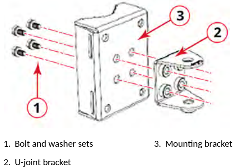
FIGURE 6 U-Joint Bracket Attached Horizontally to the Mounting Bracket
