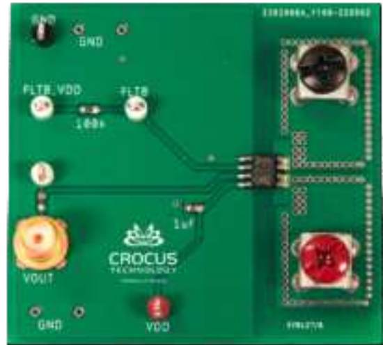
Figure 1: CT427-20AC Evaluation Board
