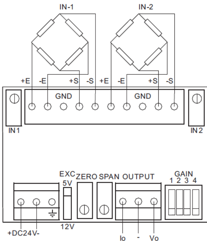
Figure 1.Connection Diagram
