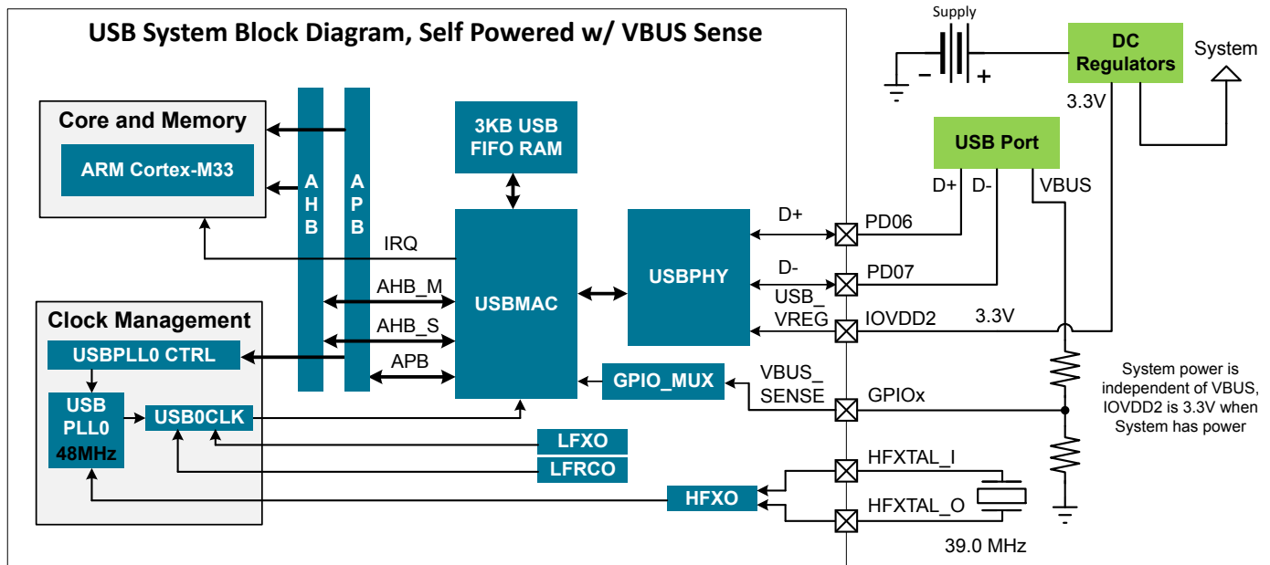
Figure 31.2. Self-powered Device
