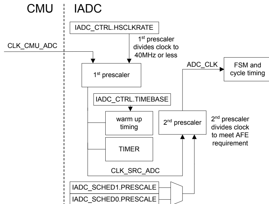
Figure 23.2. Clocking
