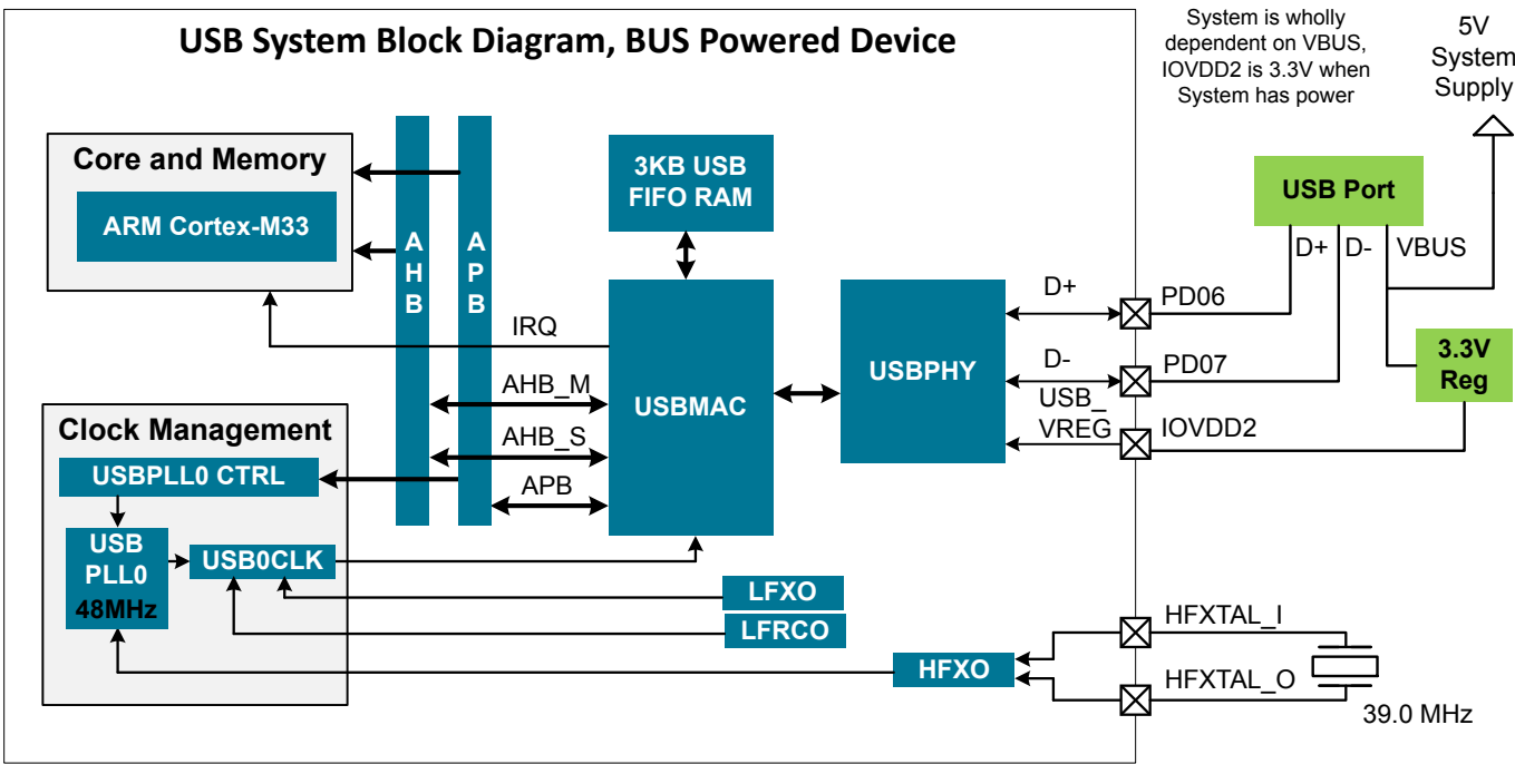
Figure 31.1. Bus-powered Device
