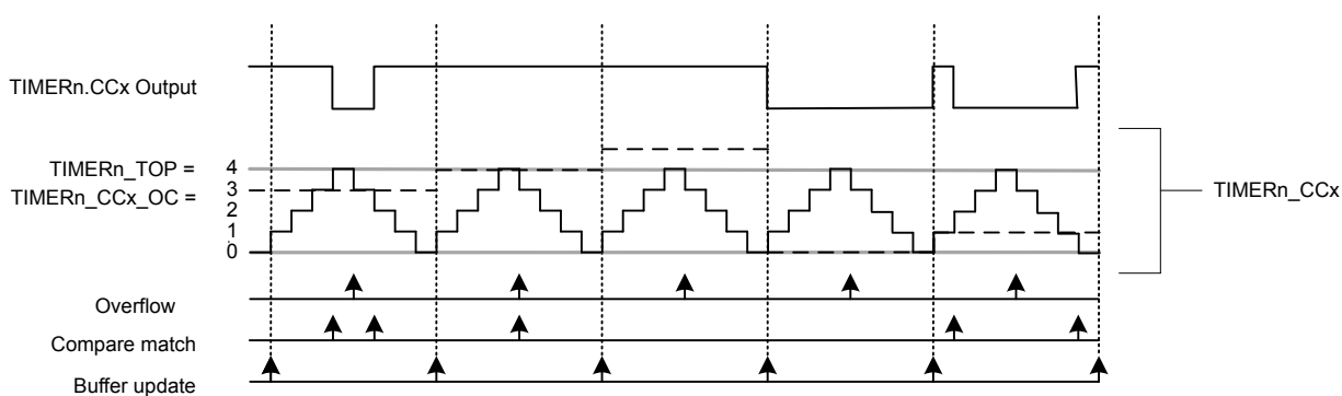
Figure 20.33. TIMER Up/Down-count PWM Generation
