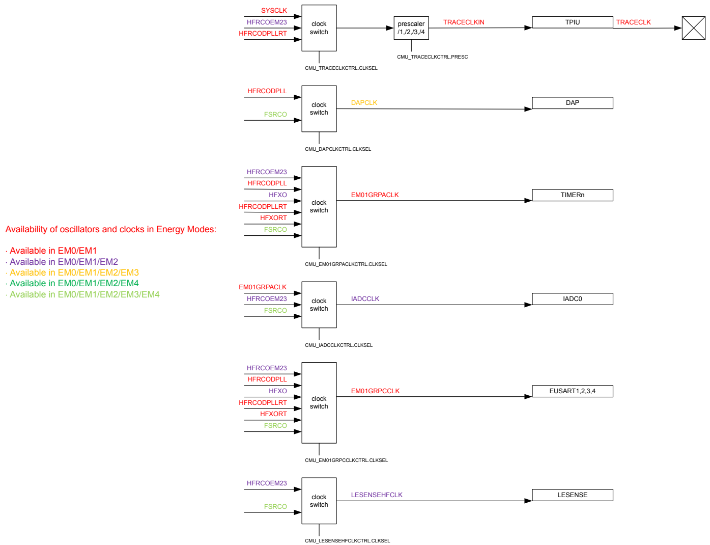
Figure 8.2. High Frequency Peripheral Clocks
