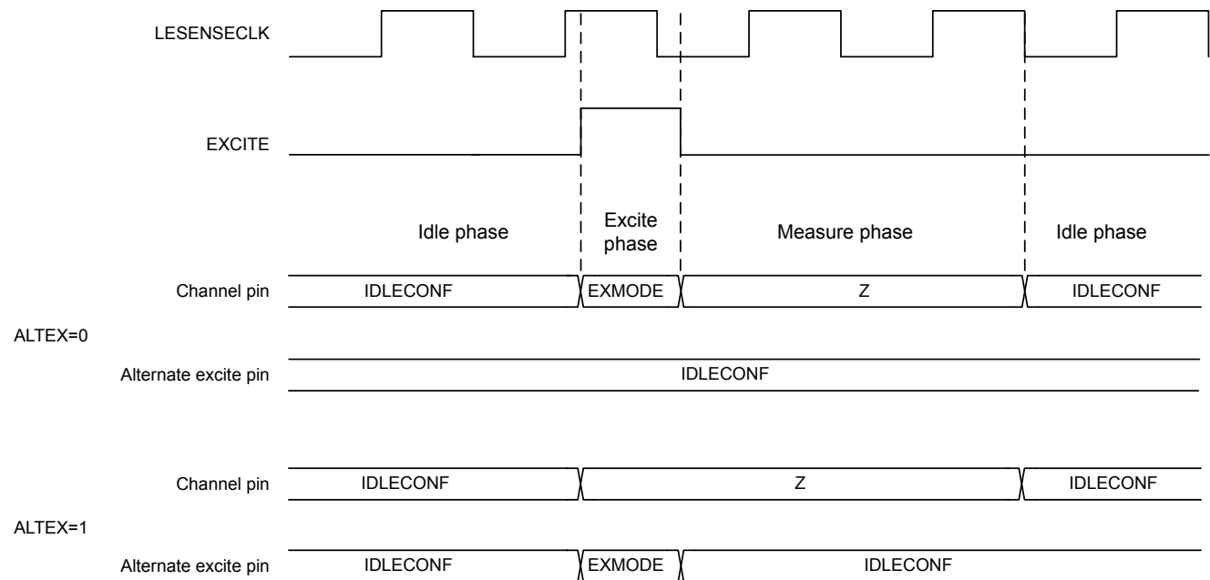
Figure 28.7. Pin Sequencing
