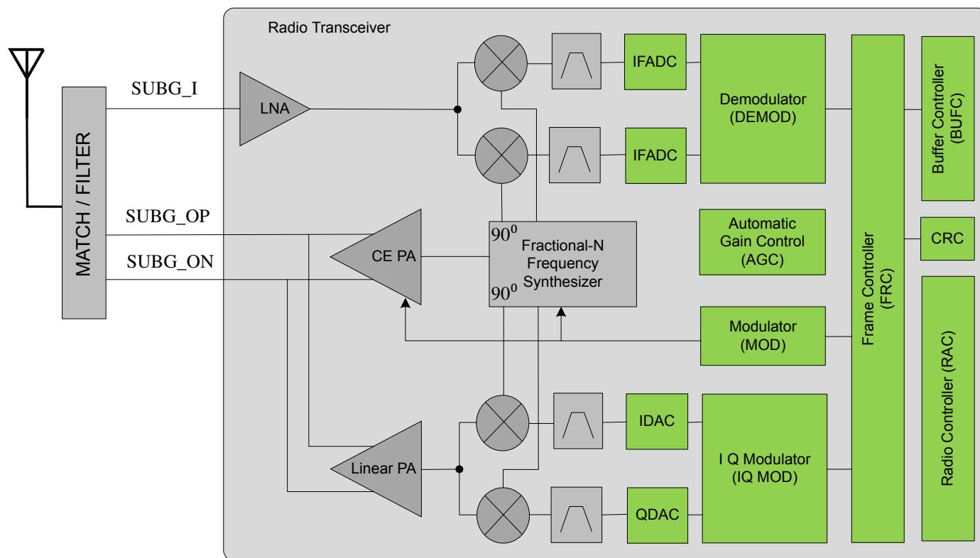
Figure 5.1. Radio Overview
