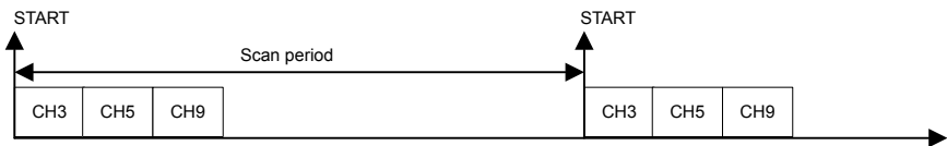
Figure 28.3. Scan Sequence
