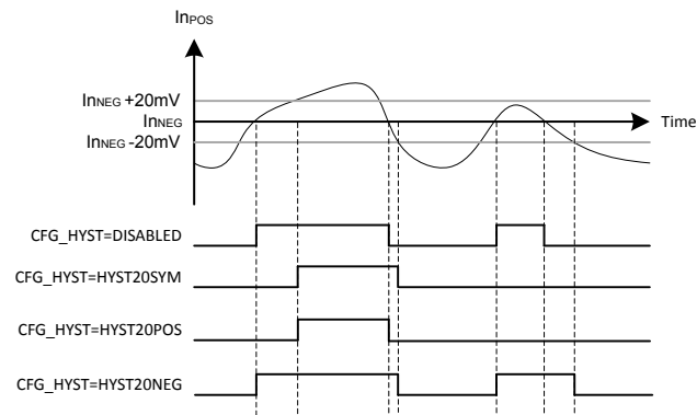
Figure 30.2. Hysteresis
