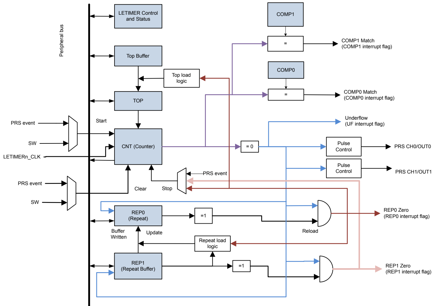
Figure 19.1. LETIMER Overview
