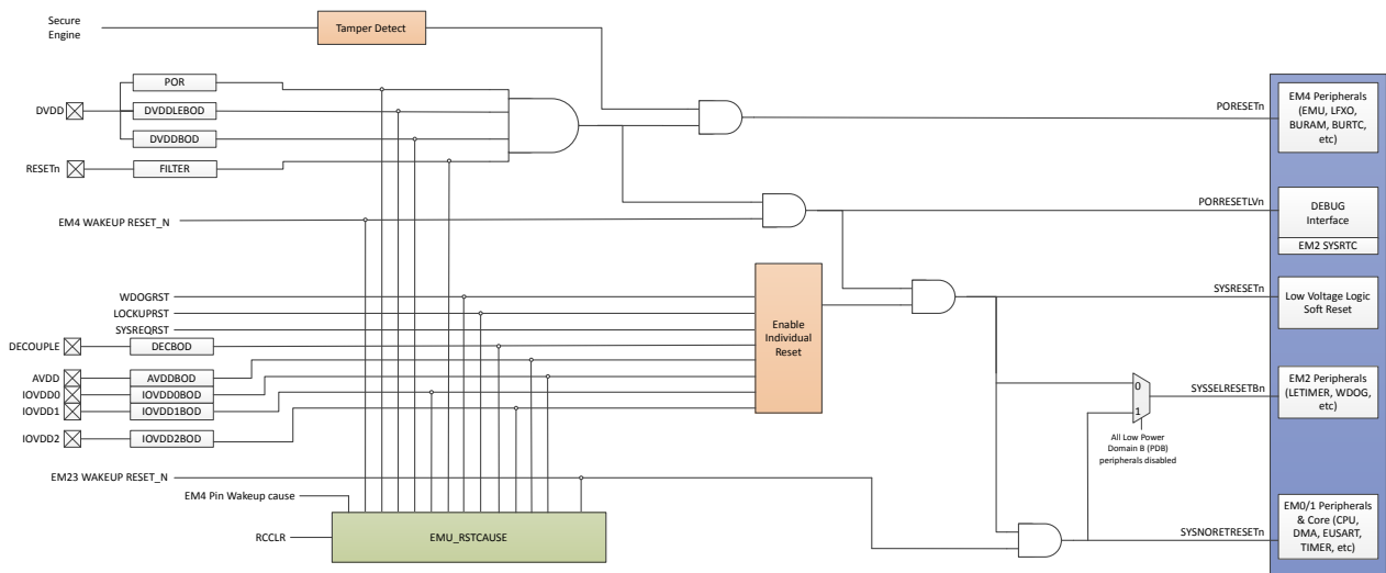
Figure 13.6. Reset Tree
