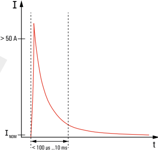
Exemplary inrush current curve
