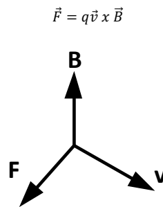
Figure 1. Lorentz force
