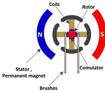
Figure 15. Brushed DC motor
