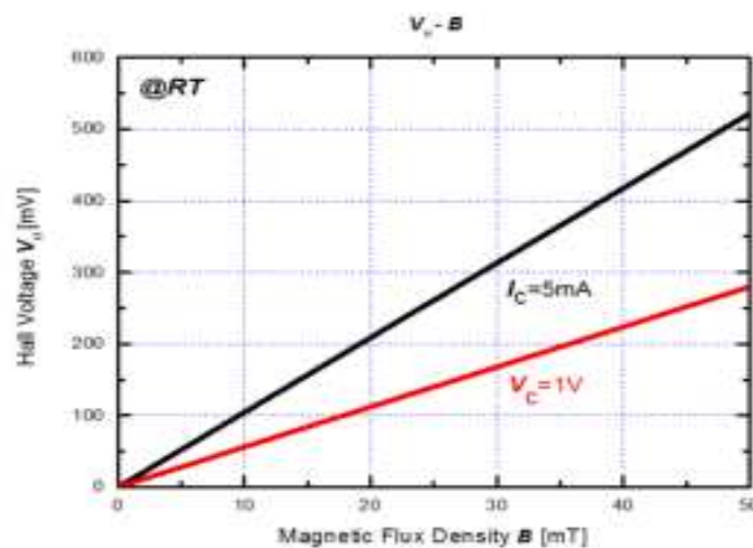
Figure 5. Hall voltage ( V_H ) as a function of magnetic flux density ( B )
