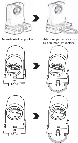
Figure showing how to convert a non-shunted lampholder to a shunted lamp holder using a jumper wire.
