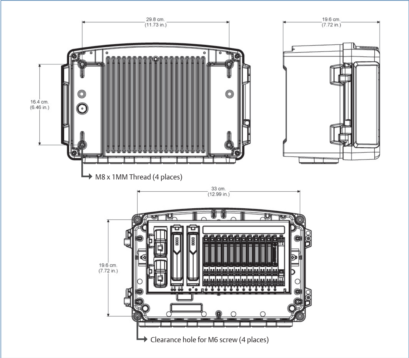
12 CHARM I/O Junction Box with Mounting holes.
