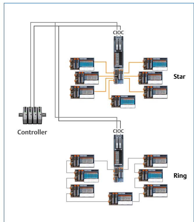
Distributed CHARMs with CHARM I/O Gateway and a mix of CHARM I/O Blocks and IS CHARM I/O Blocks. Star topology (top). Fault tolerant ring topology (bottom).
