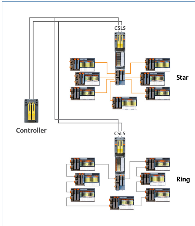
Distributed CHARMs architecture with DeltaV SIS with Electronic Marshalling.
