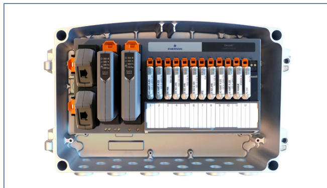
Inside view of 12 CHARM I/O Junction Box with CHARMs, it provides for easy termination close to field devices.
