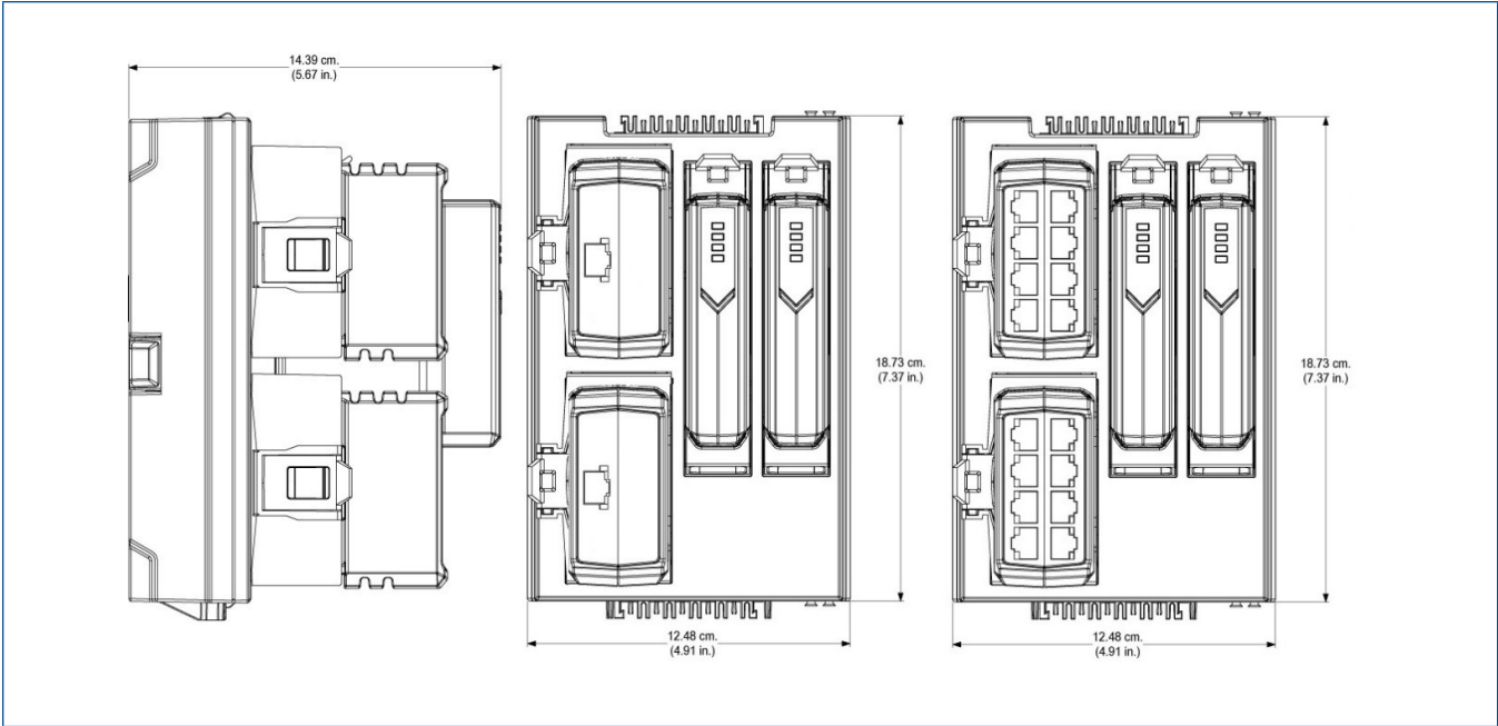
CHARM I/O Gateway with redundant Scanner Modules and redundant 1-port (center) and 8-port (right) IOPs.
