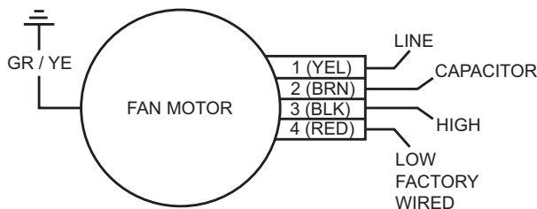
Figure 28: Size 048 (208-230/60/1 and 208-230/60/3) factory wired for low speed
