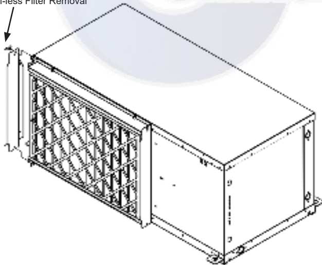
Figure 10: Optional 2" (51mm) Filter Rack/Return Air Duct Collar
