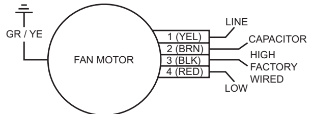
Figure 31: Sizes 060 (208-230/60/1 and (208-230/60/3)
