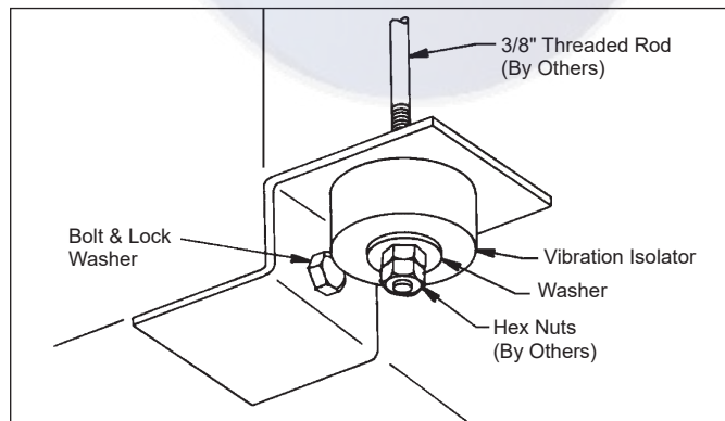
Figure 1: Hanger Bracket Detail - Sizes 007 Through 060
