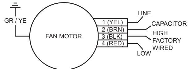
Figure 31: Sizes 060 (208-230/60/1 and (208-230/60/3)
