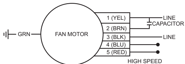
Figure 30: Size 048 (380/50/3, 460/60/3, 575/60/3) high speed
