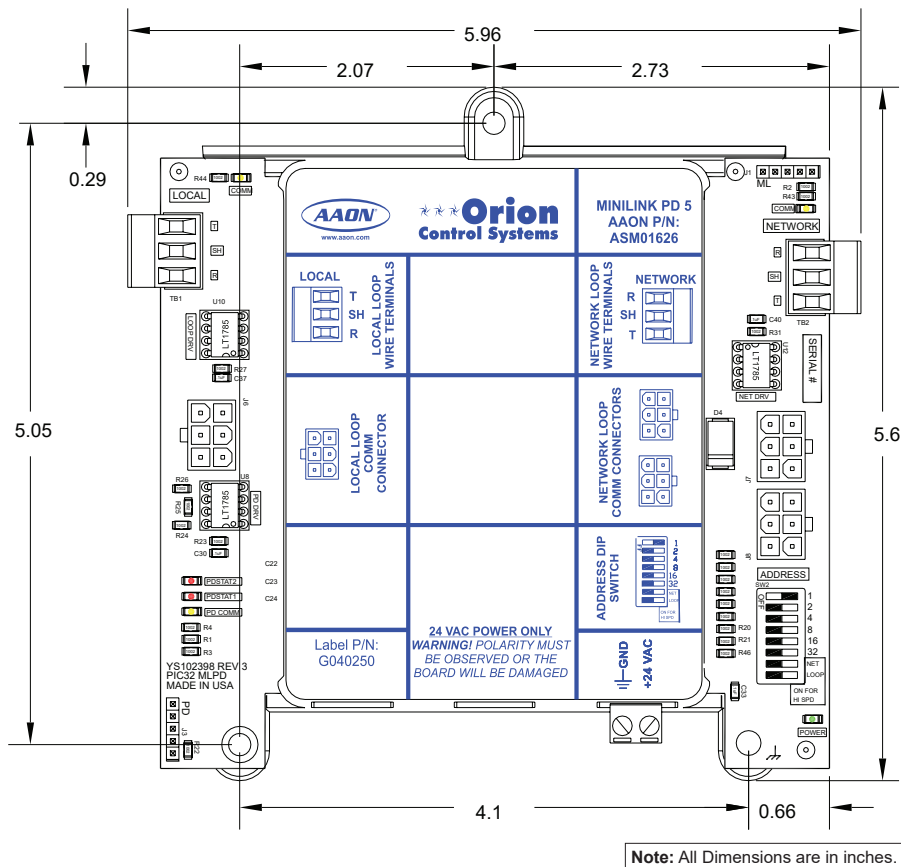
Figure 1: MiniLink PD 5 Dimensions
