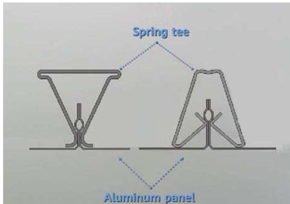
Figure 2-103 Two typical structures of spring tee ceilings
