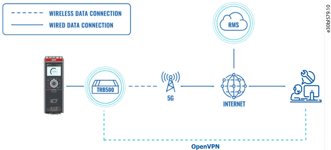
Figure 2: Network Architecture
