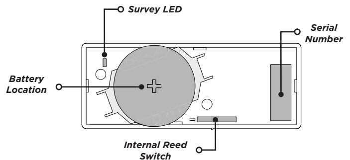
Figure 2: Battery Location and PCB Features
