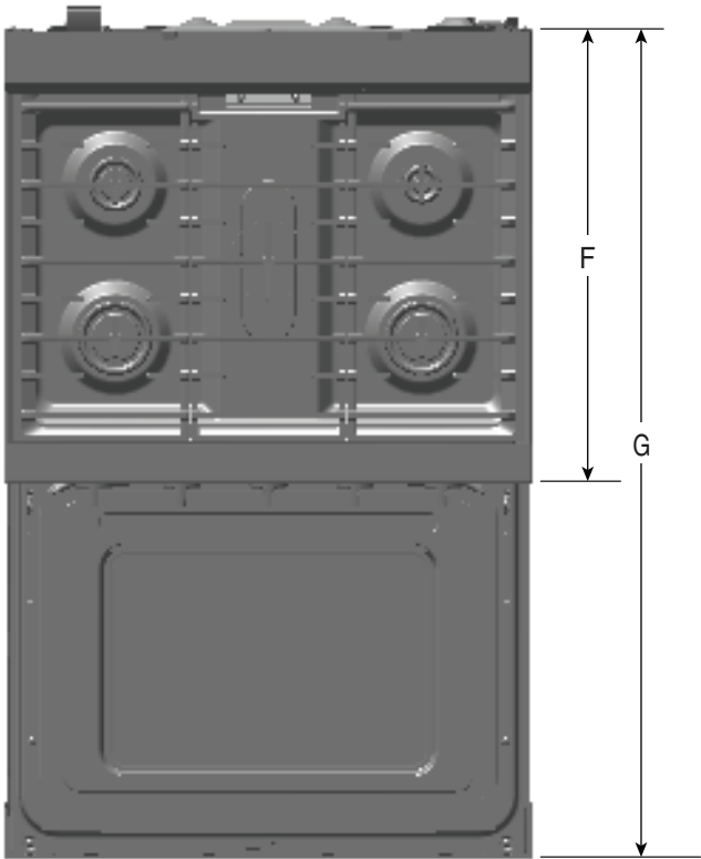
TOP VIEW
