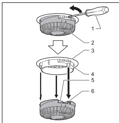
► 1. Slotted screwdriver 2. Housing 3. Cover 4. Hole 5. Fan blade 6. Hook
