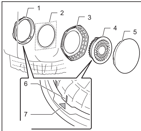
► 1. Ring 2. Hole in the jacket/vest 3. Filter attachment 4. Fan unit 5. Filter 6. "I" marking 7. Triangle marking
