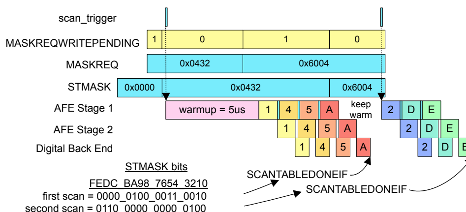
Figure 24.16. MASKREQ Updates
