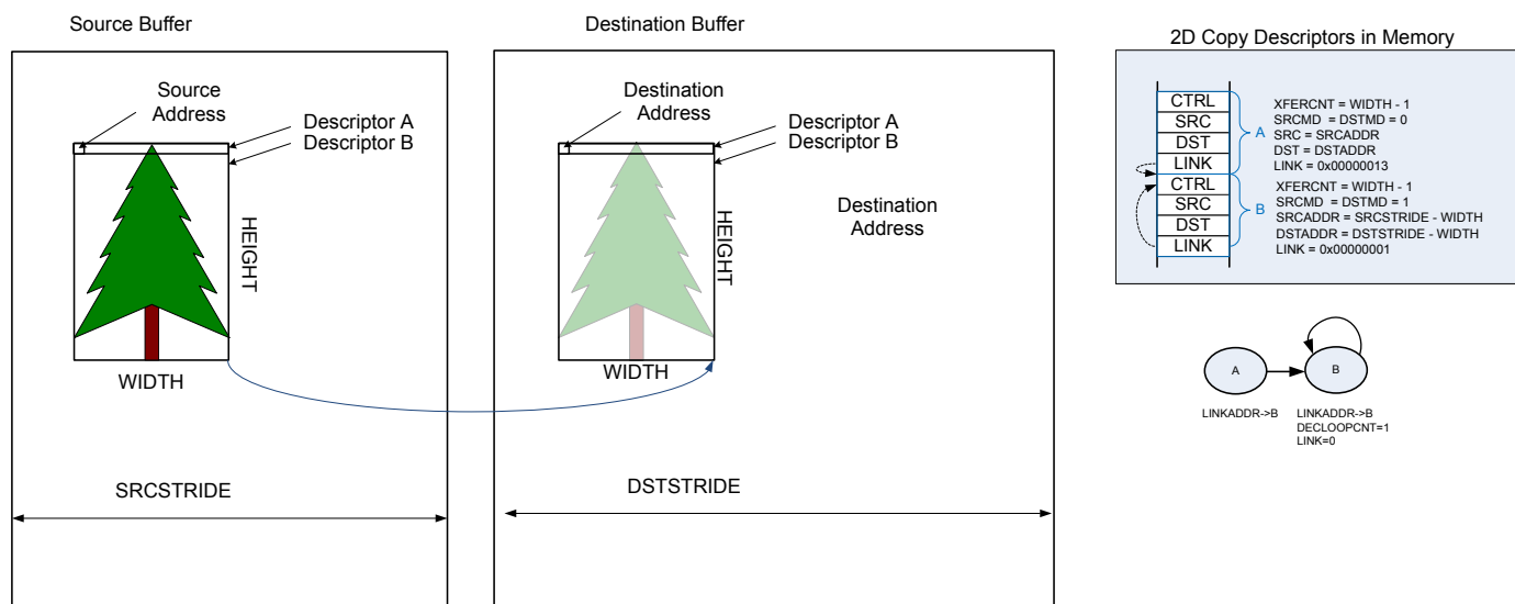
Figure 27.9. 2D Copy
