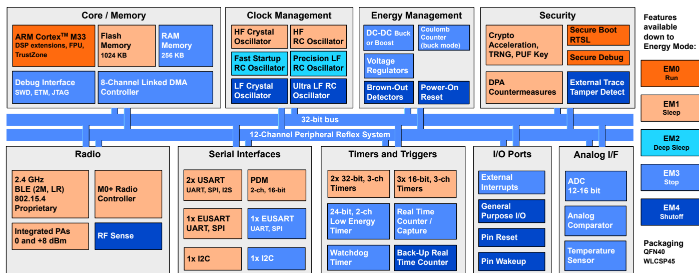
Figure 2.1. EFR32xG29 System-On-Chip Block Diagram
