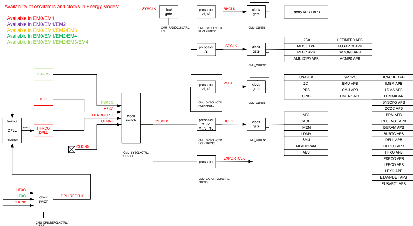
Figure 8.1. Bus Clocks
