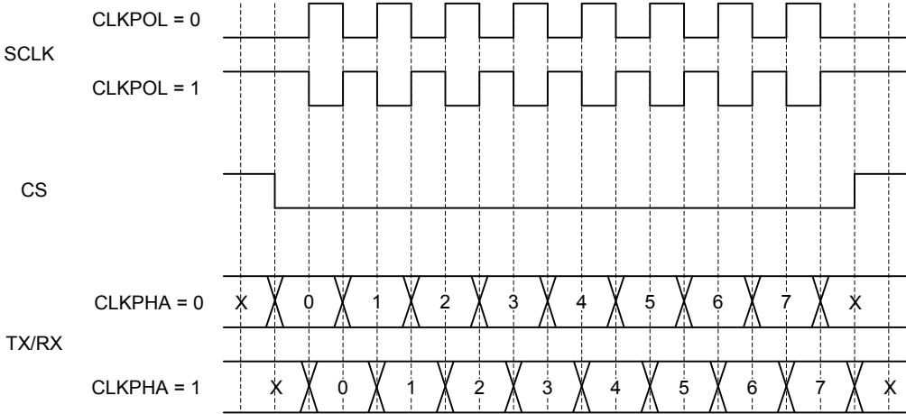
Figure 22.16. EUSART SPI Timing
