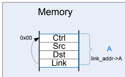
Figure 27.6. Single Descriptor Looped Transfer
