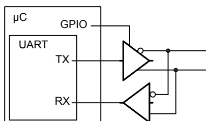
Figure 22.12. EUSART Half Duplex Communication with External Driver
