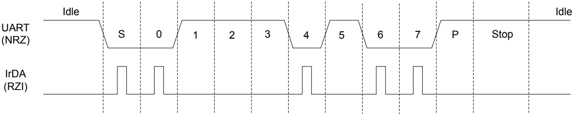
Figure 22.13. EUSART Example RZI Signal for a given EUSART Frame
