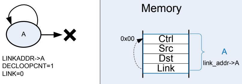
Figure 27.6. Single Descriptor Looped Transfer
