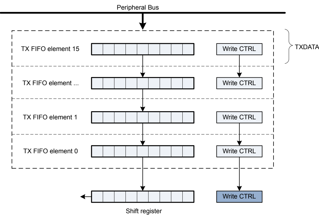
Figure 22.6. Transmit FIFO Operation
