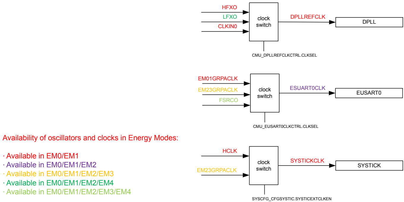
Figure 8.4. Mixed Frequency Peripheral Clocks
