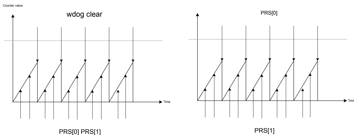
Figure 28.3. PRS Edge Monitoring in WDOG
