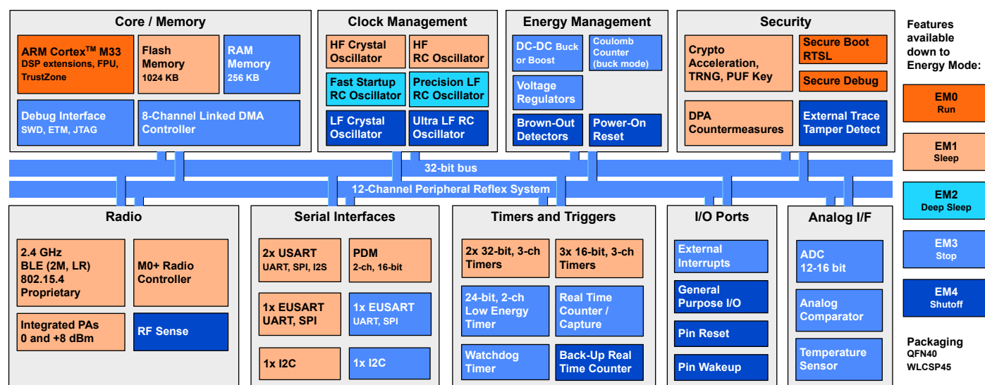
Figure 2.1. EFR32xG29 System-On-Chip Block Diagram
