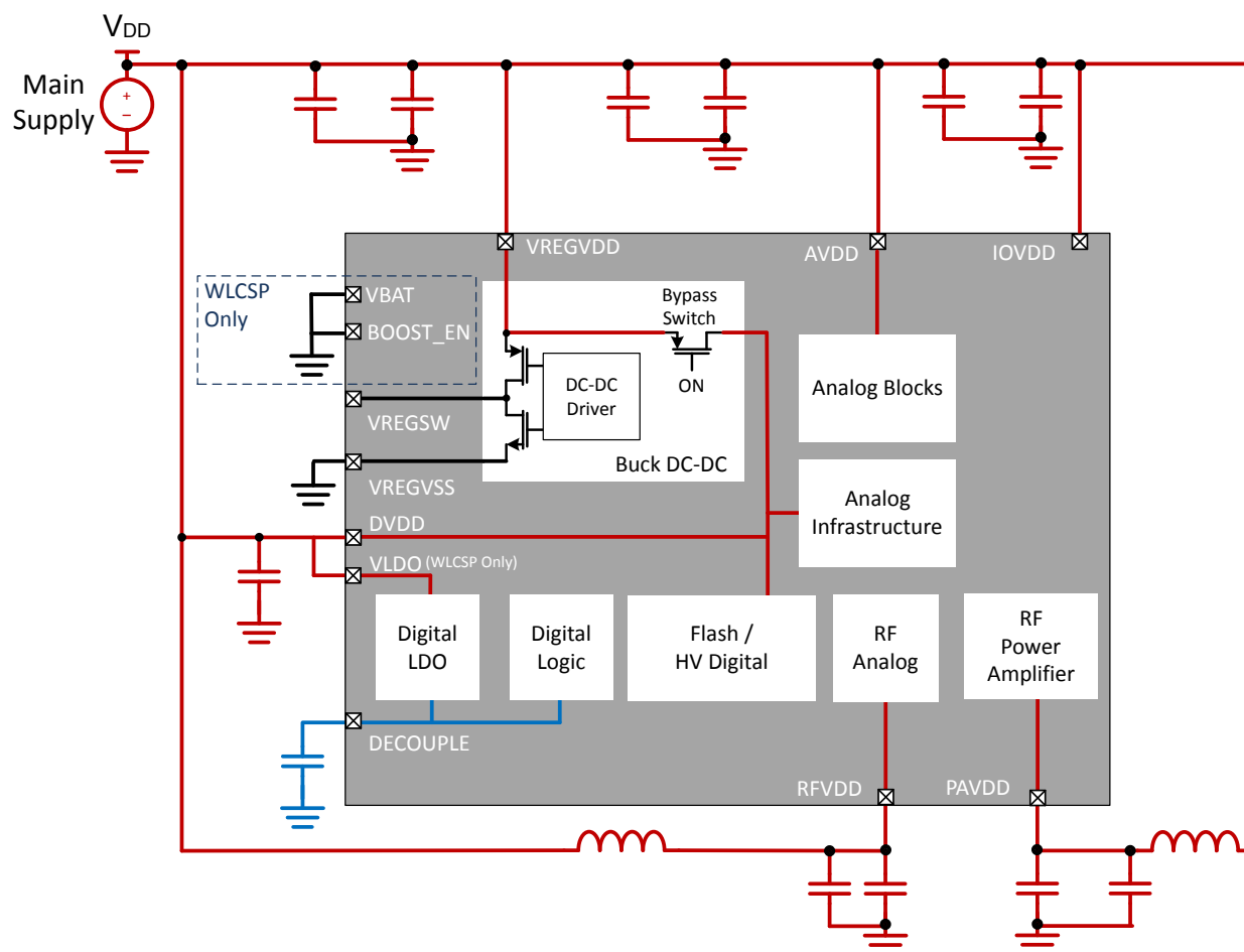
Figure 12.2. DC-DC Off Power Configuration
