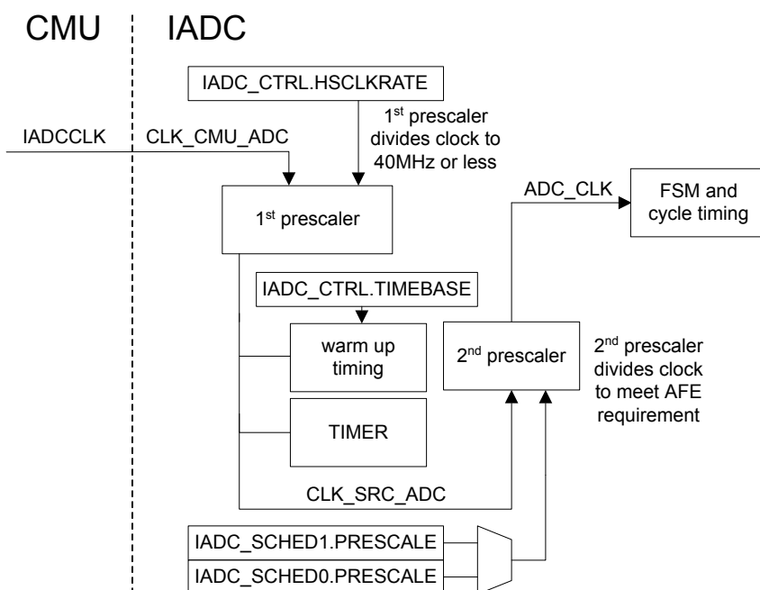
Figure 24.2. Clocking
