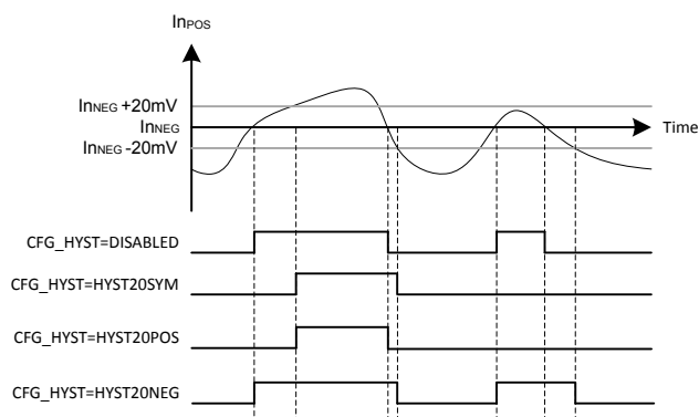
Figure 25.2. Hysteresis
