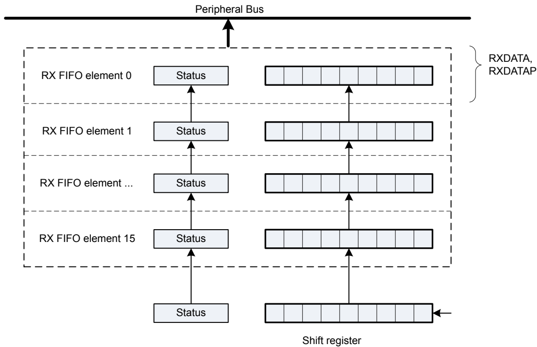
Figure 22.7. EUSART Receive FIFO Operation
