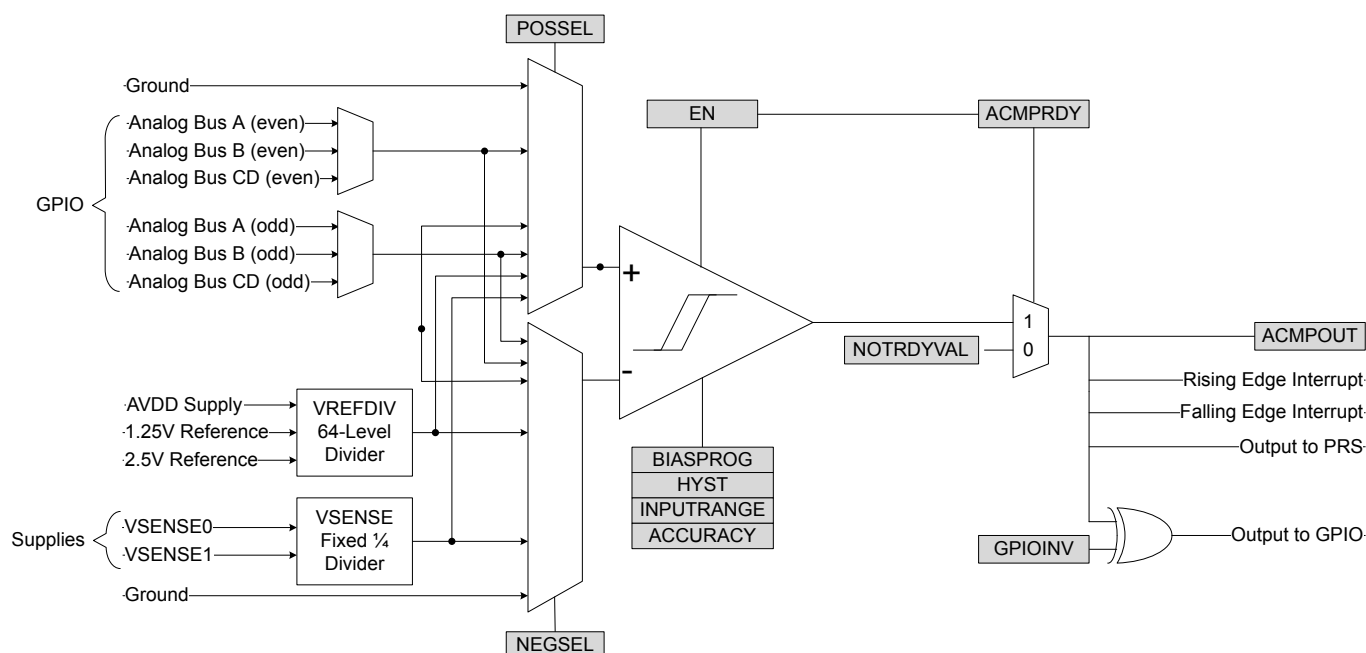
Figure 25.1. ACMP Overview
