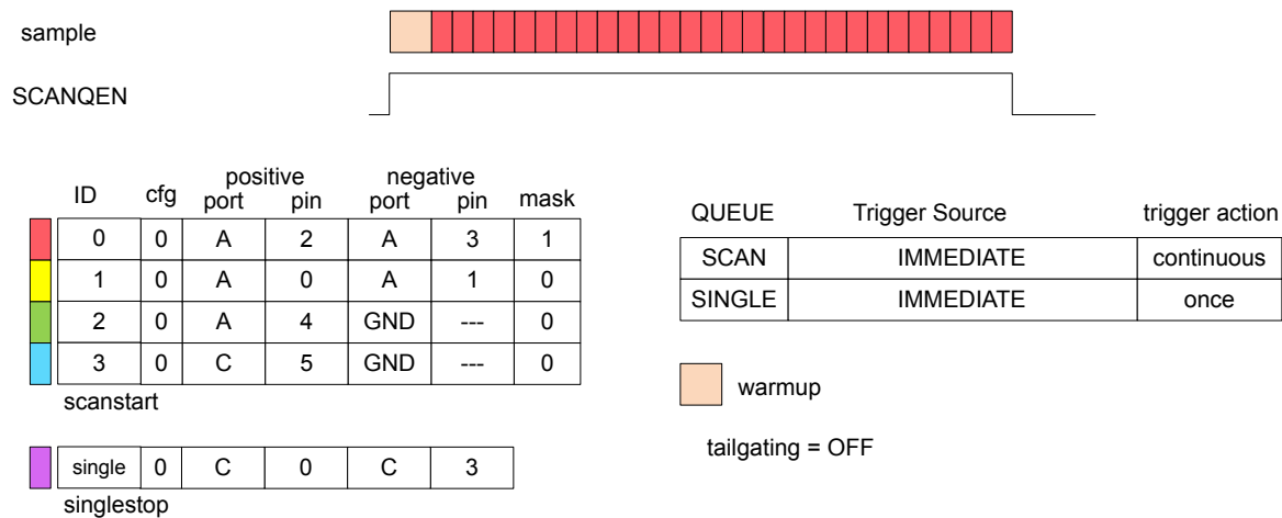
Figure 24.9. Continuous Conversions
