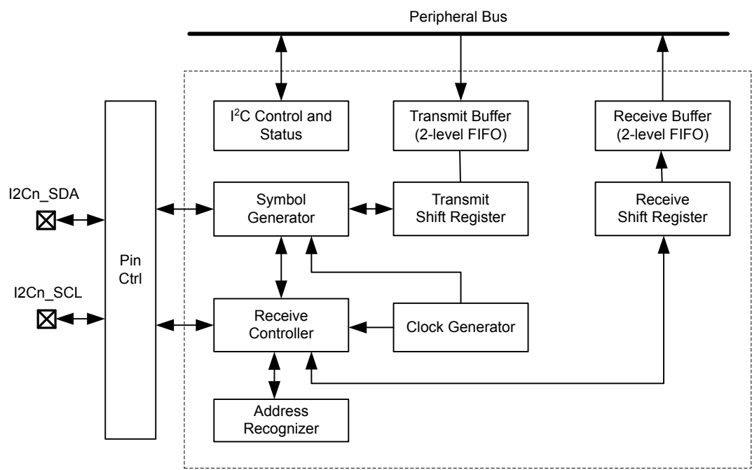
Figure 23.1. I2C Overview
