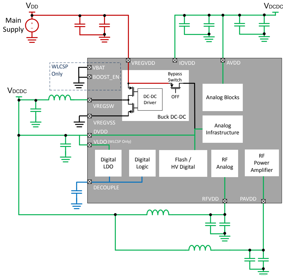
Figure 12.3. Buck DC-DC Power Configuration
