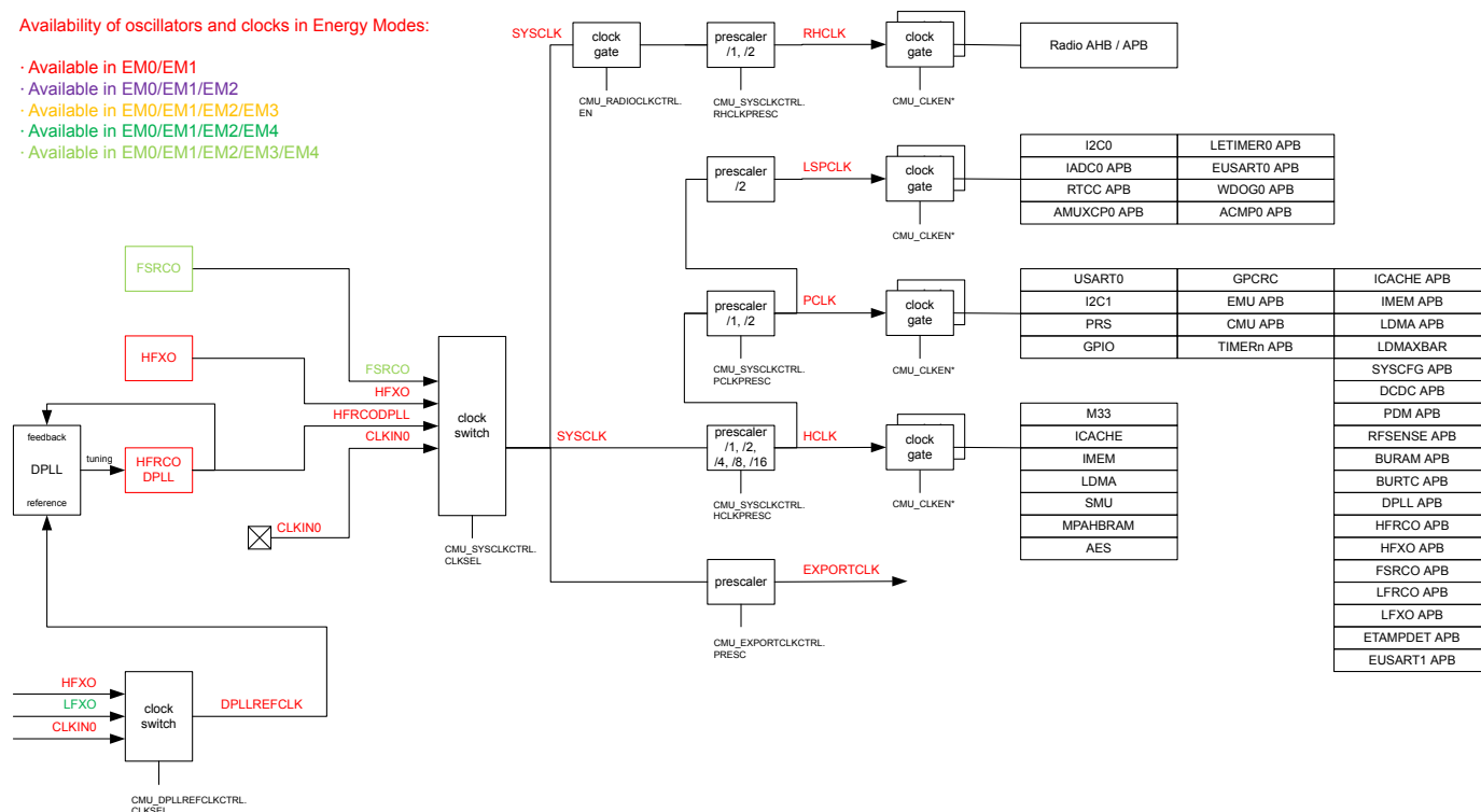
Figure 8.1. Bus Clocks
