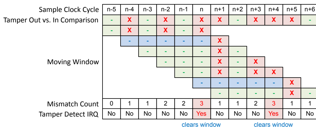
Figure 11.3. Moving Window Filter Example
