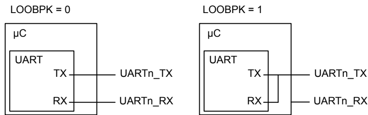
Figure 22.11. EUSART Local Loopback
