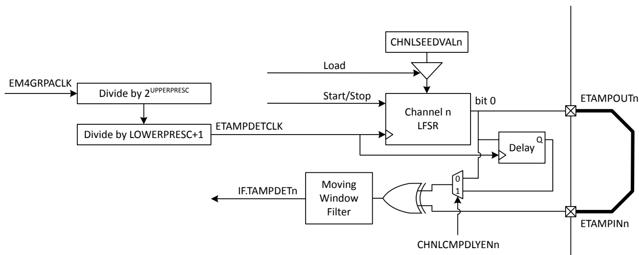
Figure 11.1. ETAMPDET Block Diagram
