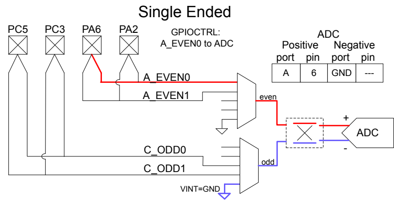
Figure 24.11. Single-Ended Port/Pin Selection Even Channel
