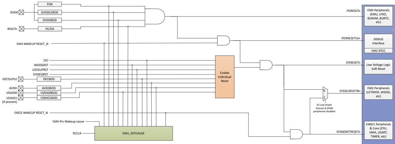
Figure 12.6. Reset Tree
