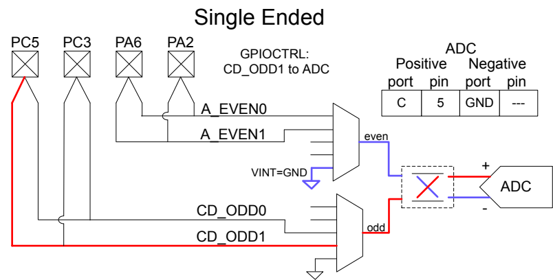
Figure 24.10. Single-Ended Port/Pin Selection Odd Channel
