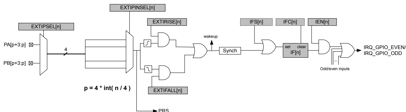
Figure 26.6. Pin n Interrupt Generation
