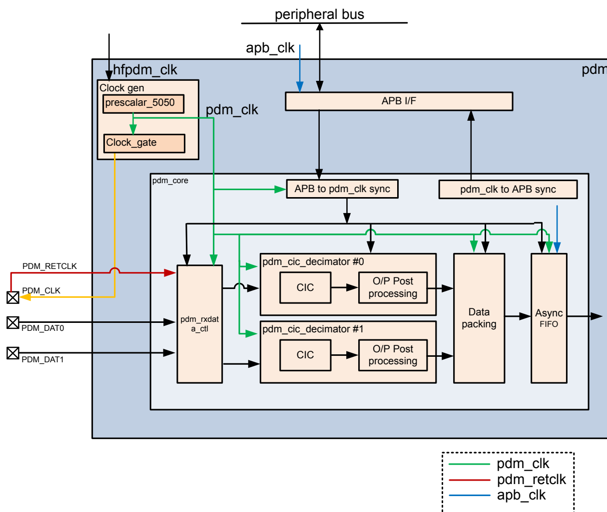
Figure 20.1. PDM Overview
