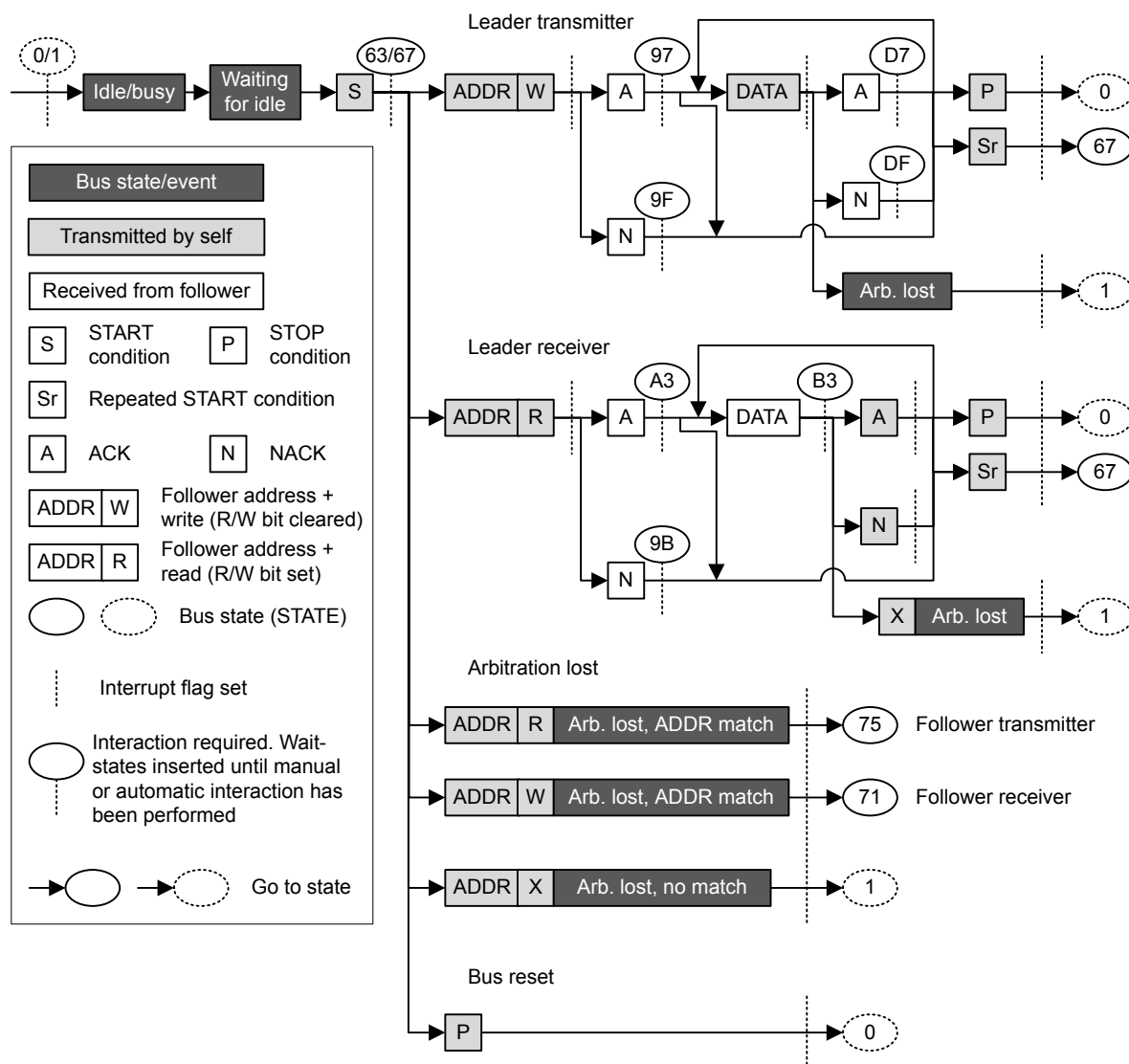
Figure 23.16. I2C Leader State Machine
