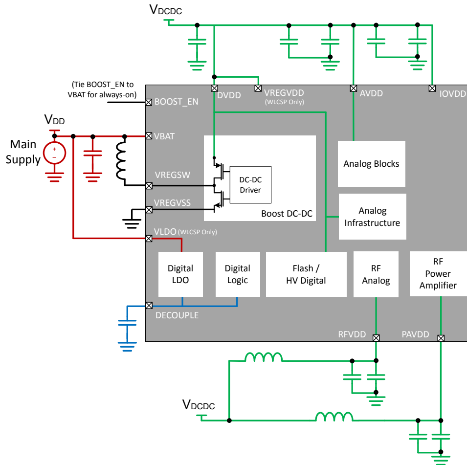
Figure 12.4. Boost DC-DC Power Configuration
