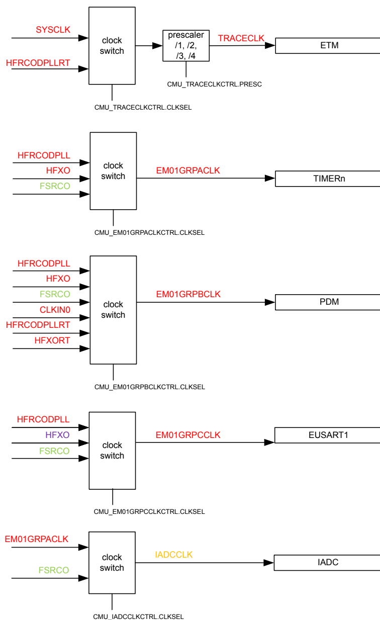
Figure 8.2. High Frequency Peripheral Clocks
