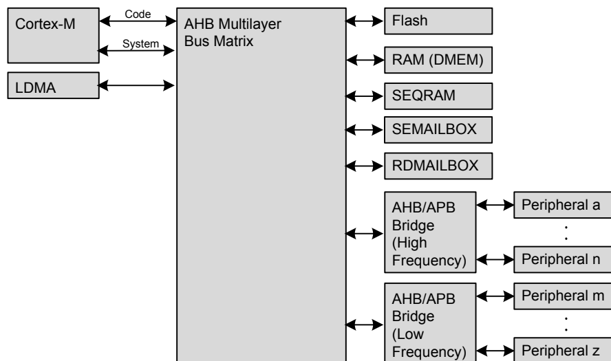
Figure 4.2. EFR32xG29 Bus System
