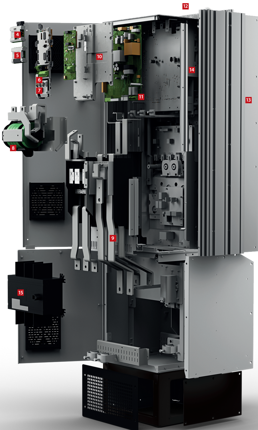
VLT® AutomationDrive FC 302, enclosure size T5
