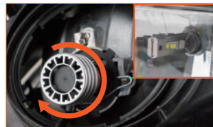
Fig. 4: Rotate the heat sink to get a better beam pattern (It will get a best beam pattern if the LED chips face 3-9 o'clock.)
