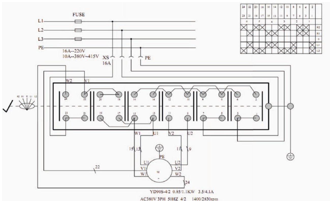
Electrical schema
