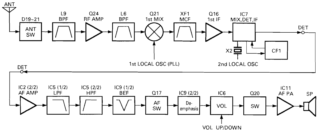
Fig. 2 Receiving system
