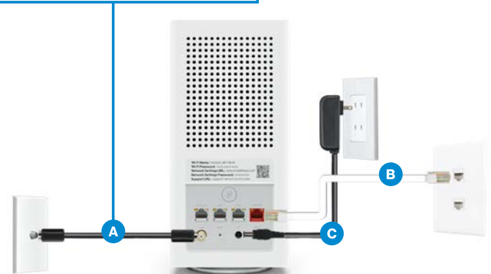
Verizon Router (Same connections for the Fios Router and Fios Quantum Gateway)
