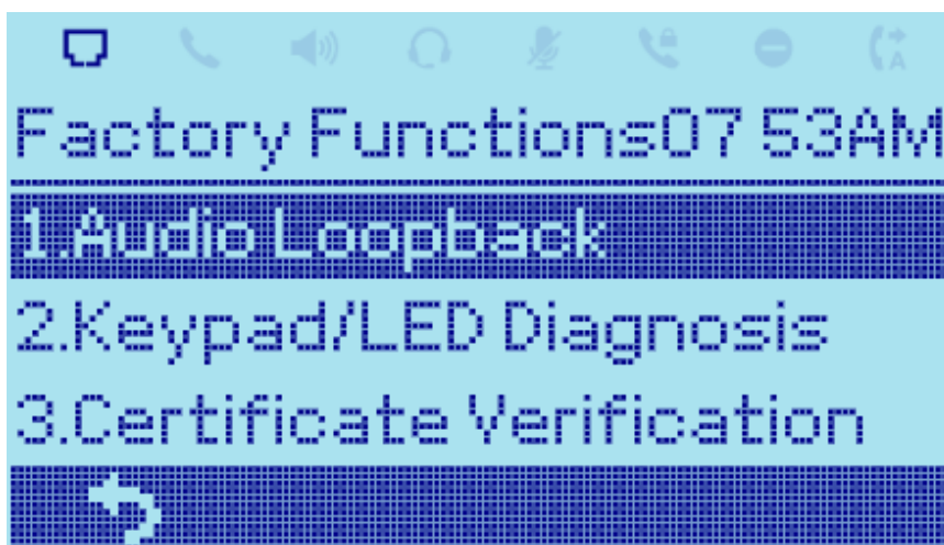
Factory Functions
