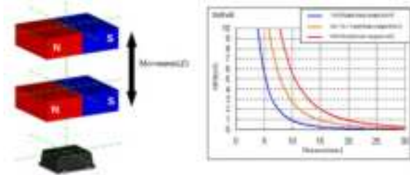
Fig.2 MFD vs vertical magnet movement
