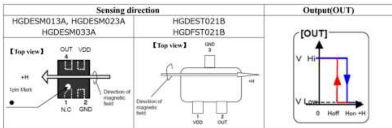
Fig.1 Sensing direction for magnetic switch
