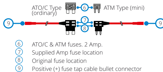
Fuse Tap Cables
