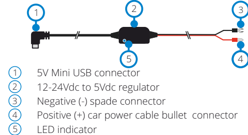
Camera Power Cable
