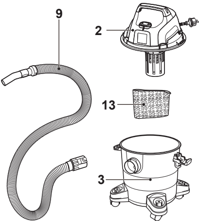
Fig. 5, Wet vacuuming
